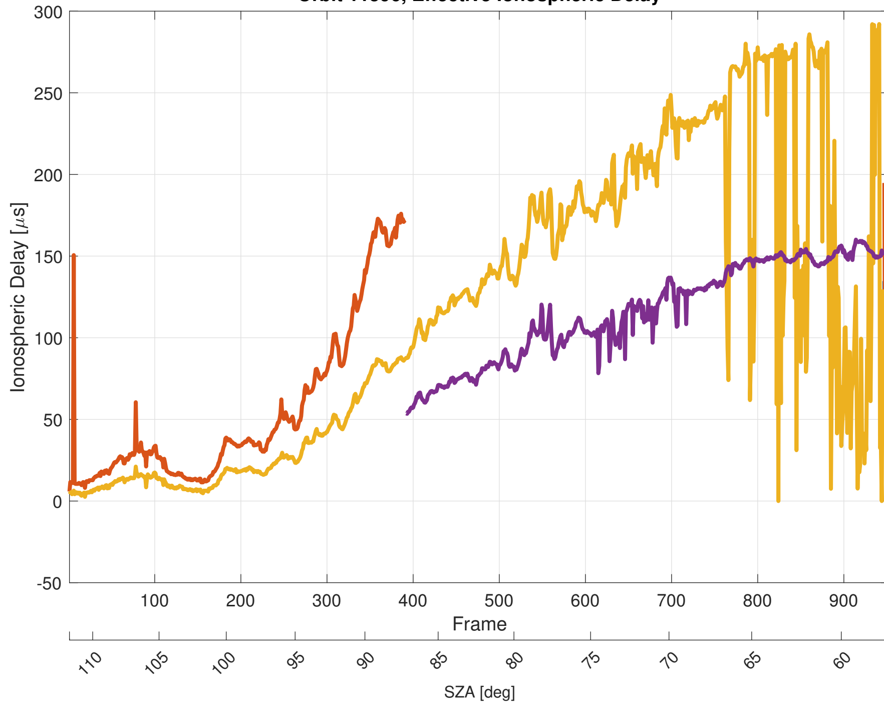
Orbit 11596, Effective Ionospheric Delay
