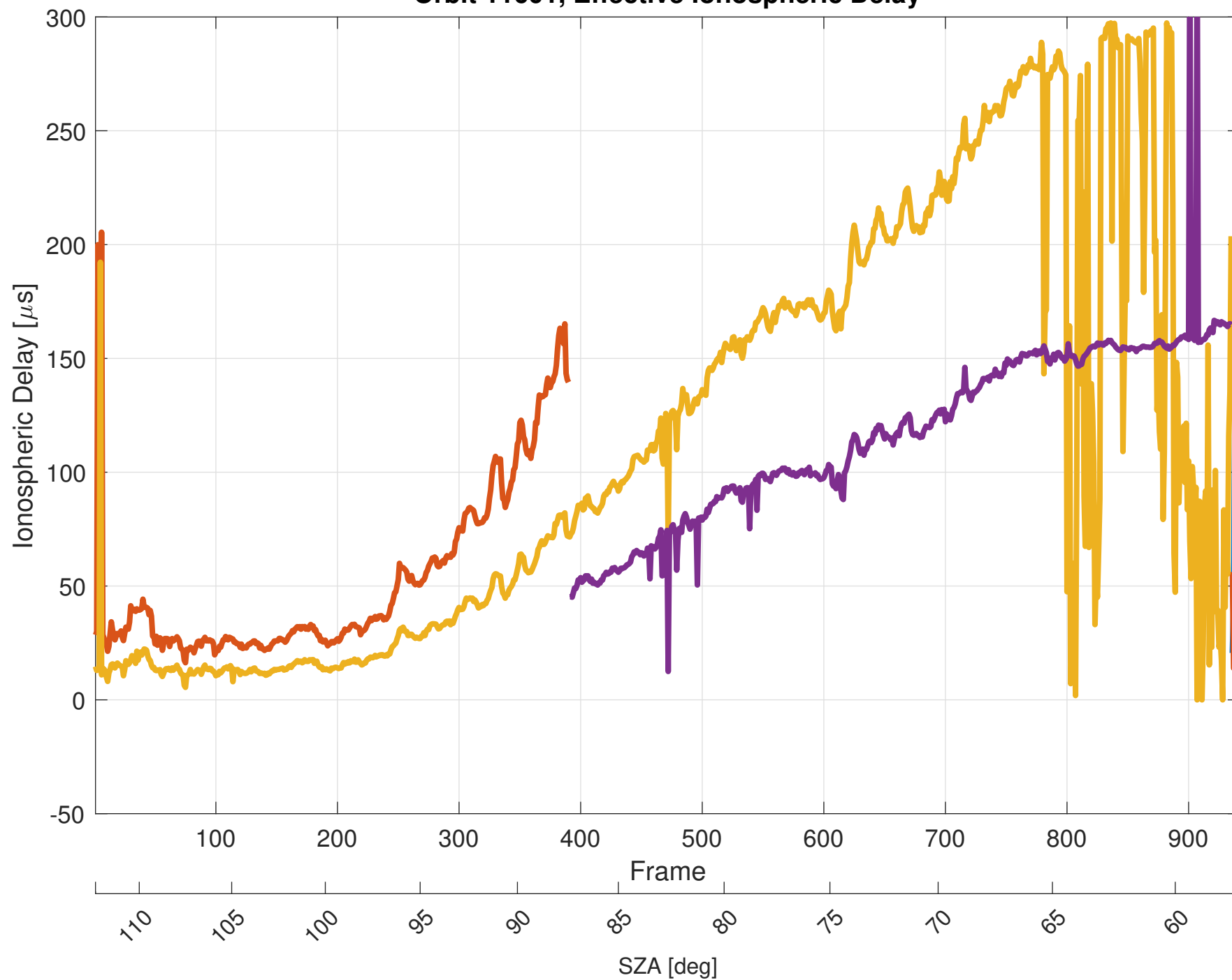
Orbit 11601, Effective Ionospheric Delay
