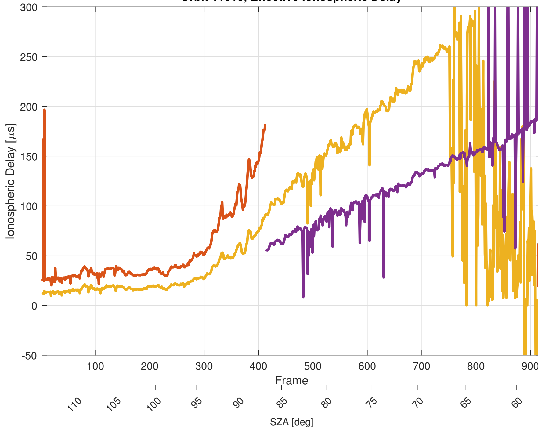
Orbit 11615, Effective Ionospheric Delay
