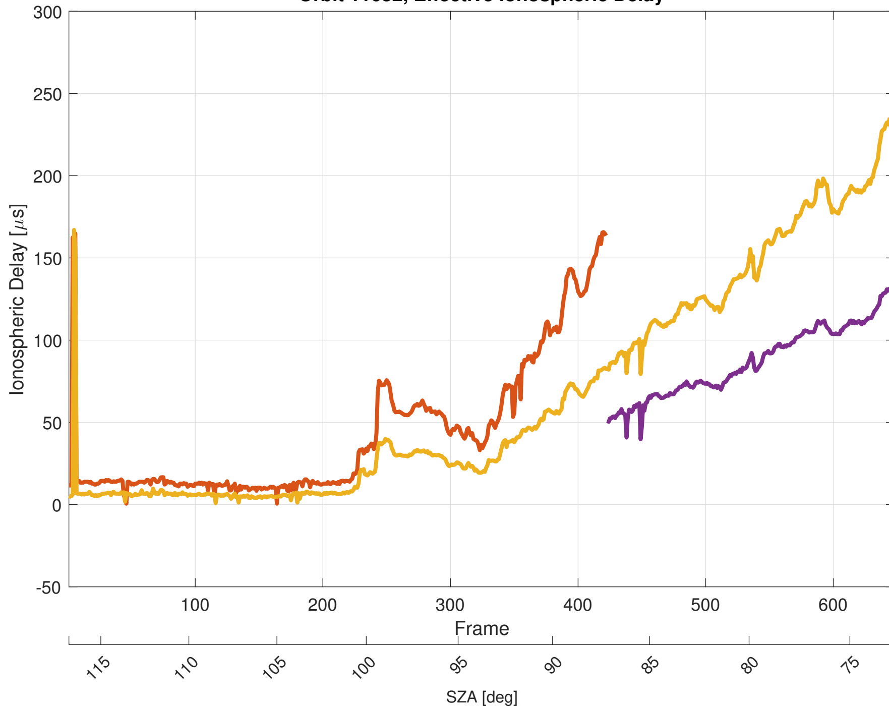
Orbit 11632, Effective Ionospheric Delay
