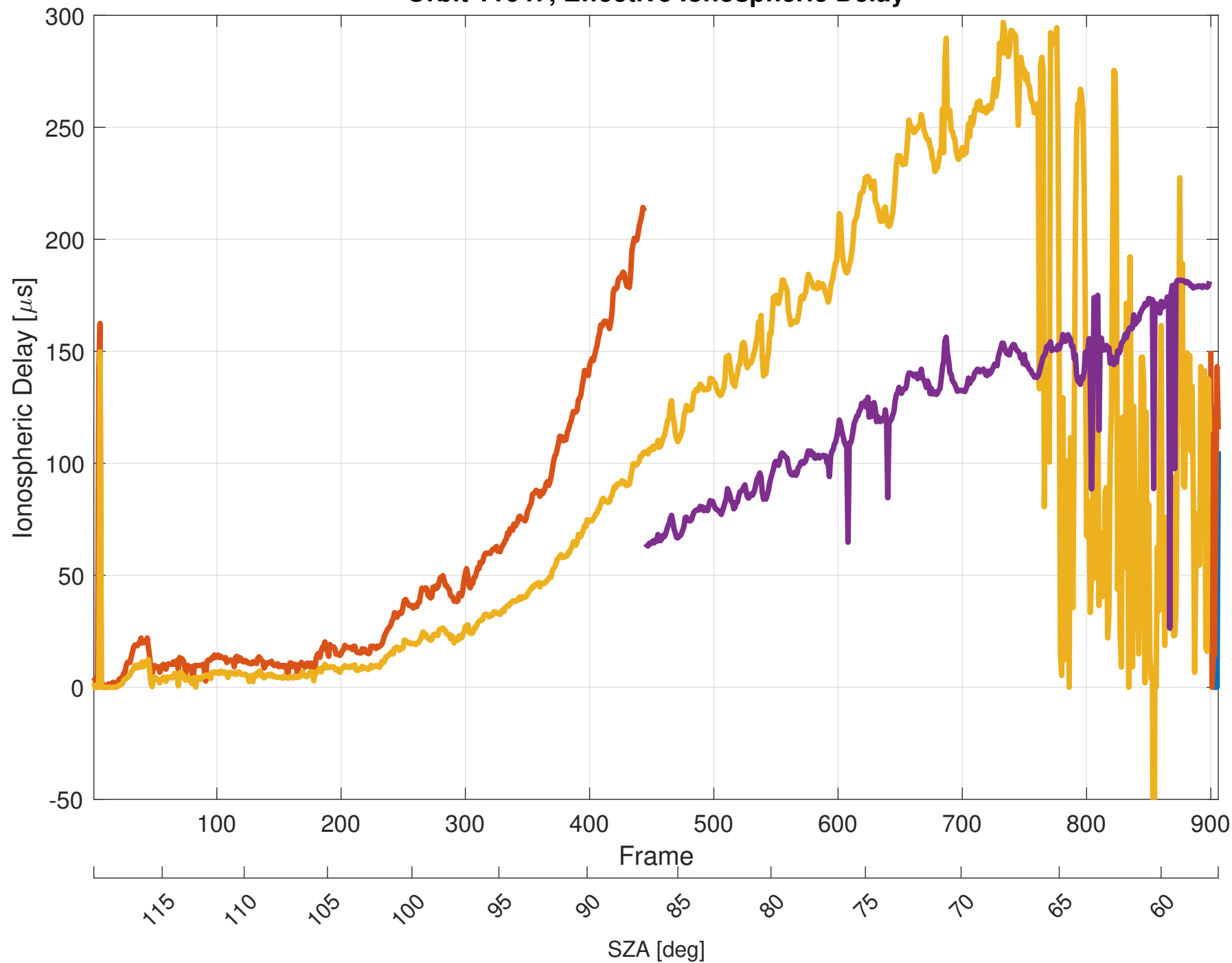
Orbit 11647, Effective Ionospheric Delay
