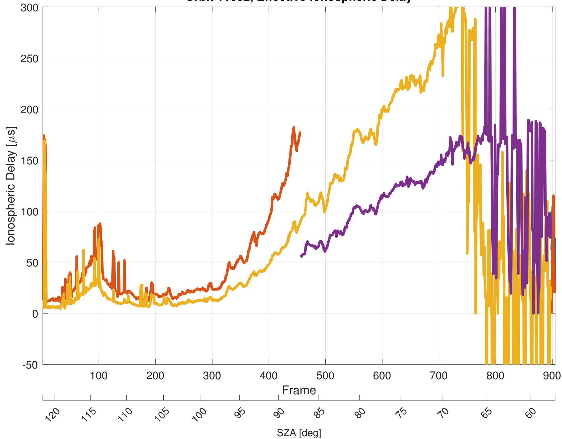
Orbit 11662, Effective Ionospheric Delay
