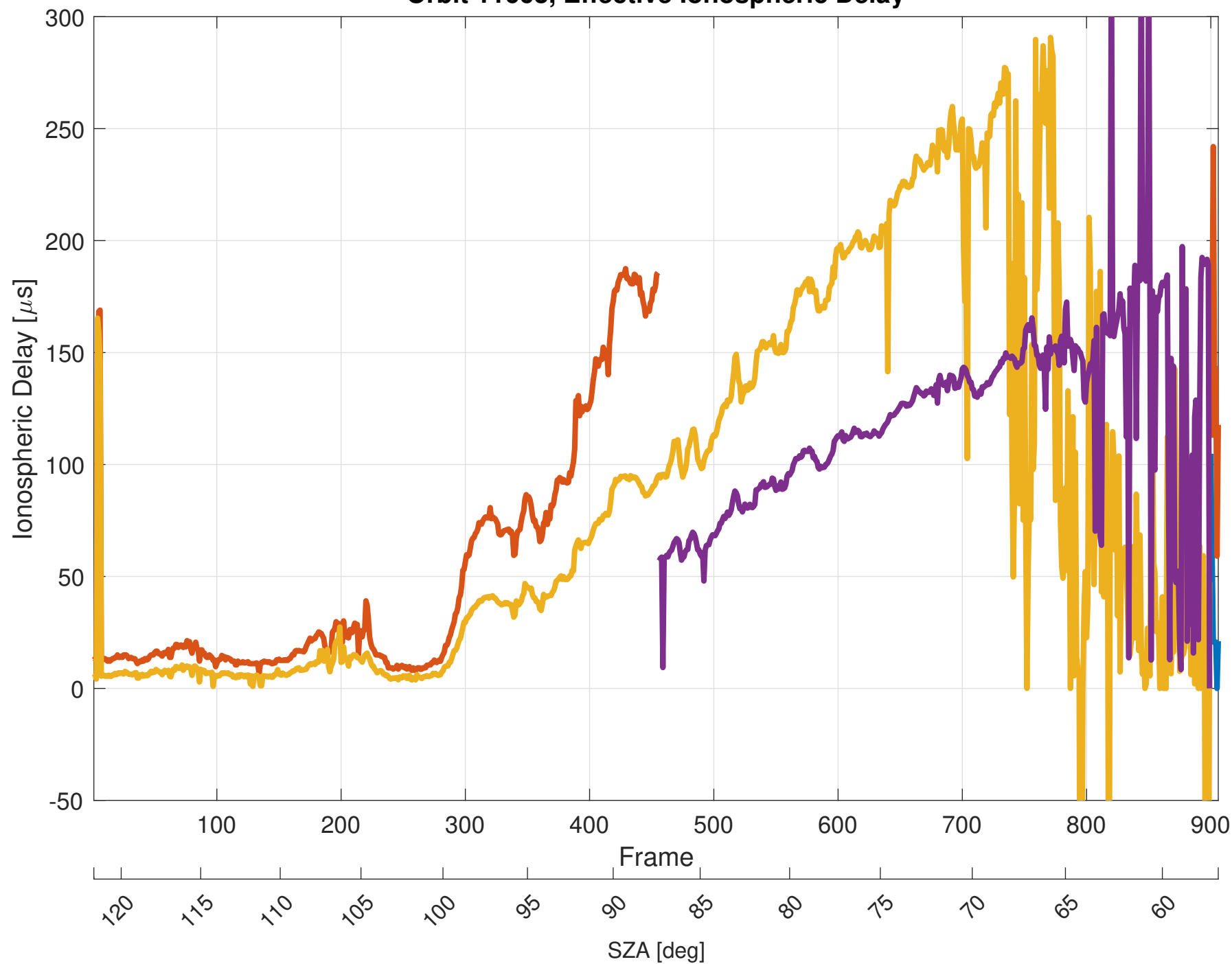
Orbit 11663, Effective Ionospheric Delay
