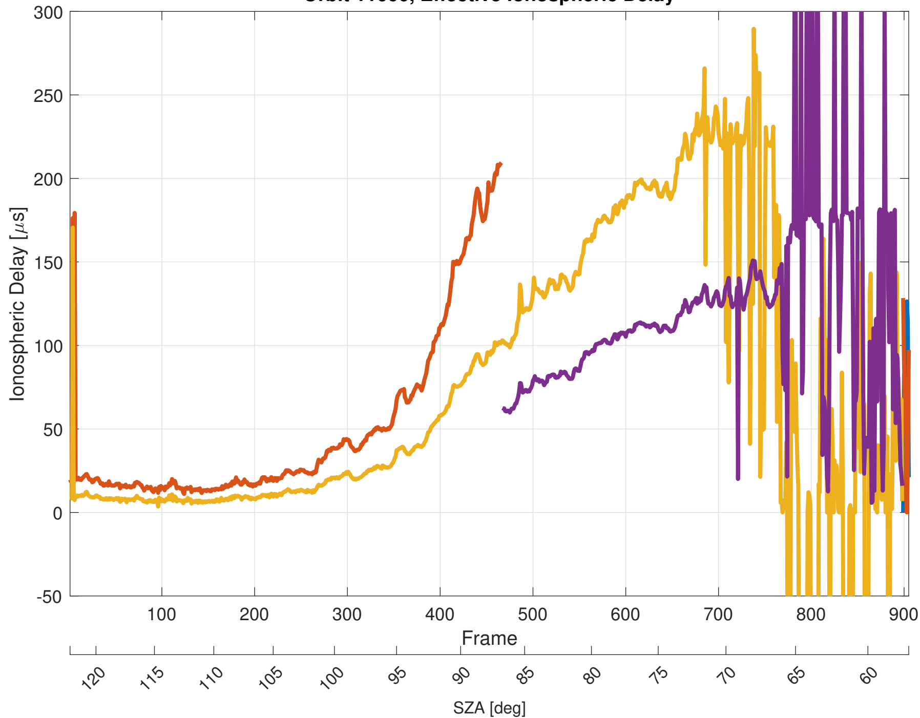
Orbit 11666, Effective Ionospheric Delay
