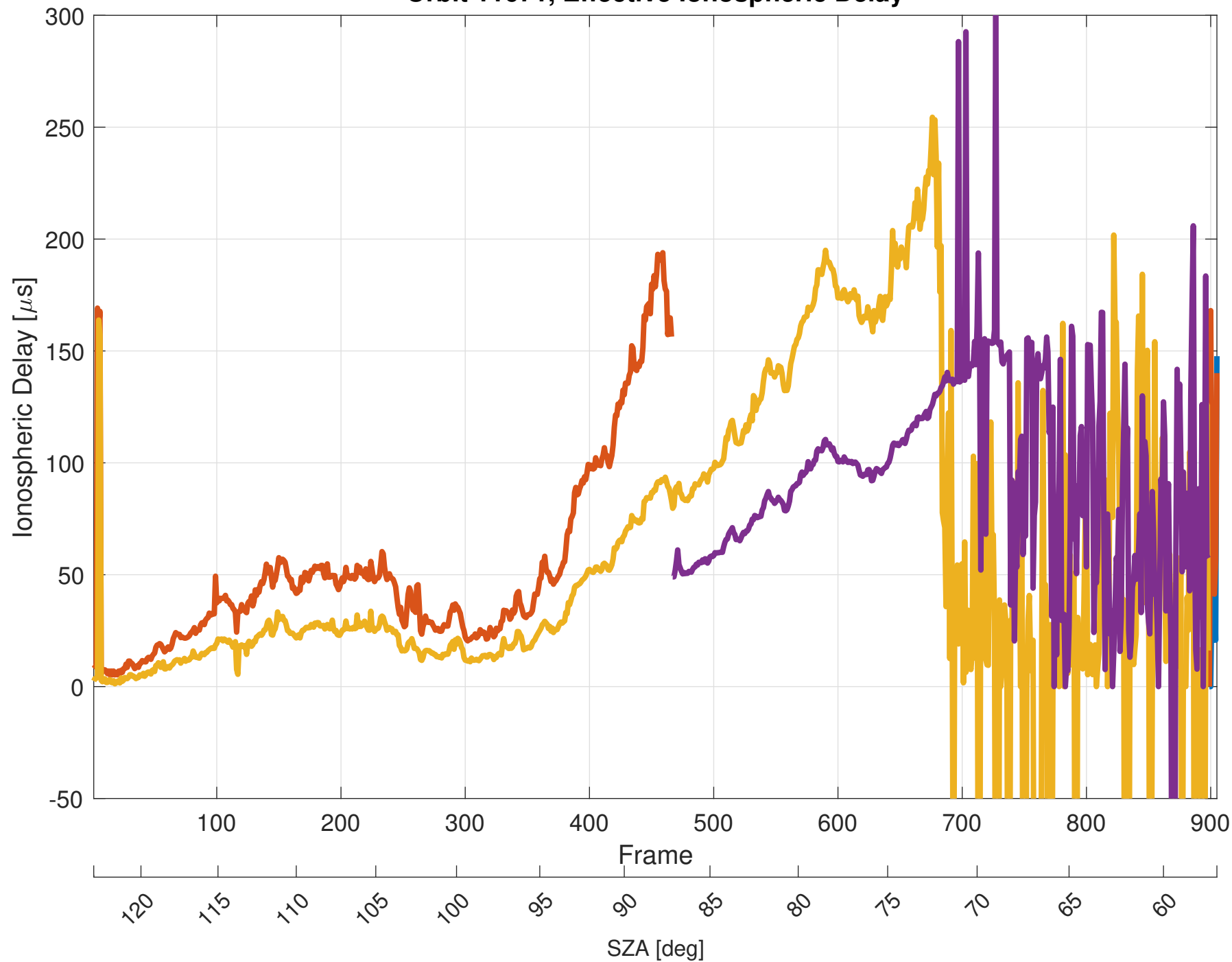
Orbit 11671, Effective Ionospheric Delay
