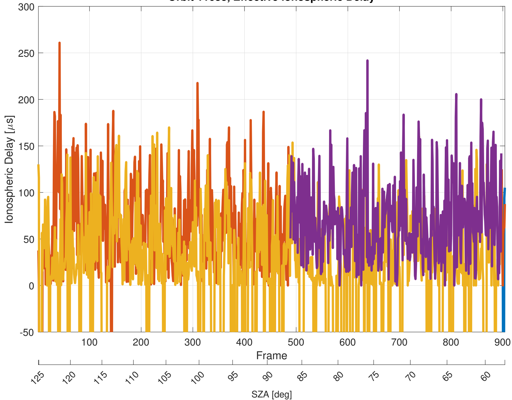
Orbit 11683, Effective Ionospheric Delay
