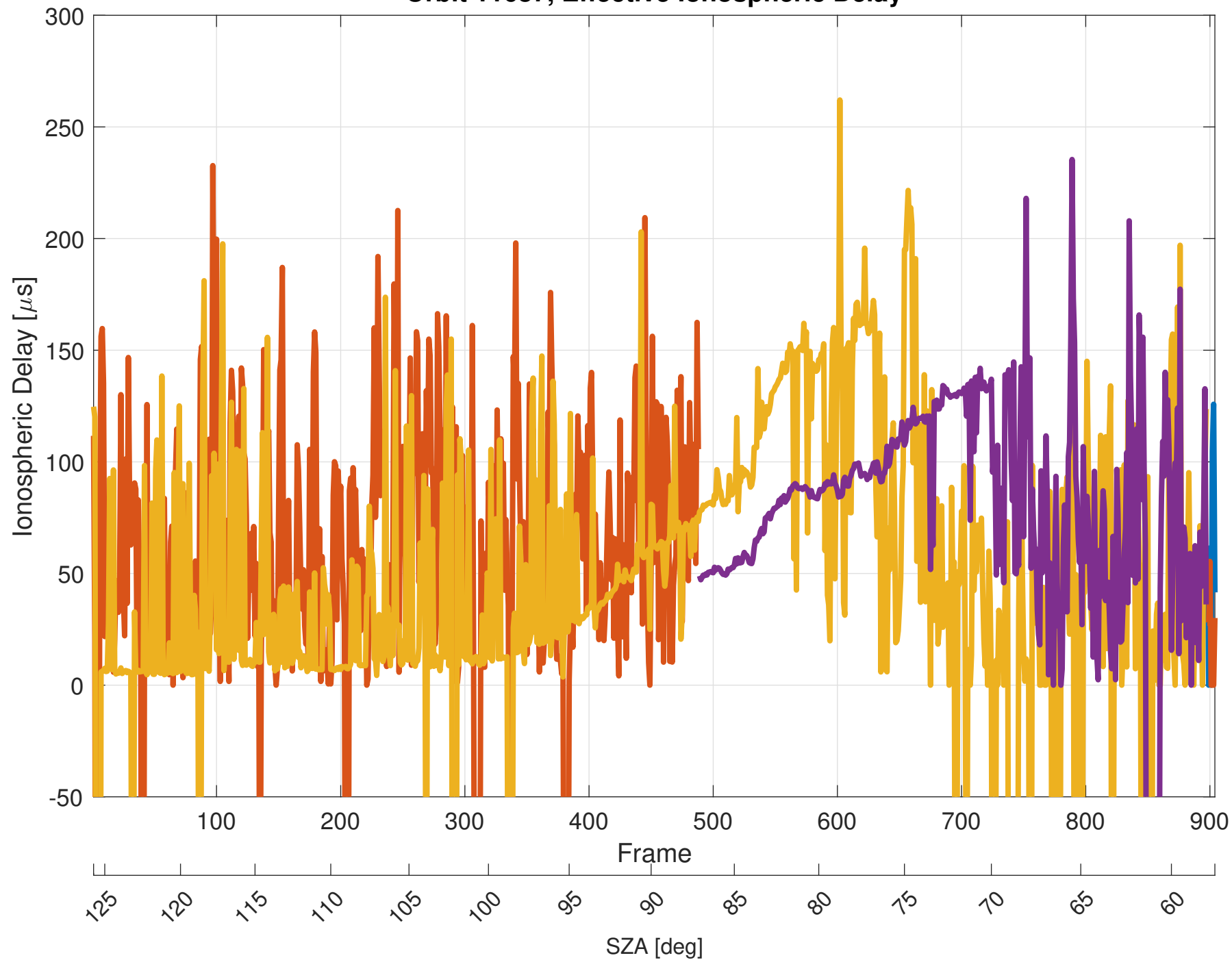
Orbit 11687, Effective Ionospheric Delay
