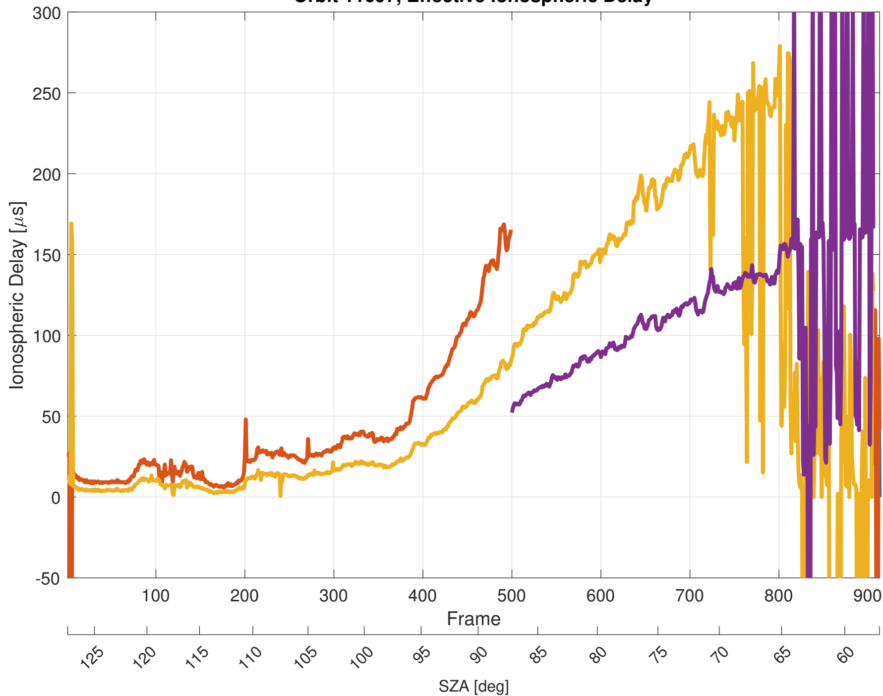
Orbit 11697, Effective Ionospheric Delay
