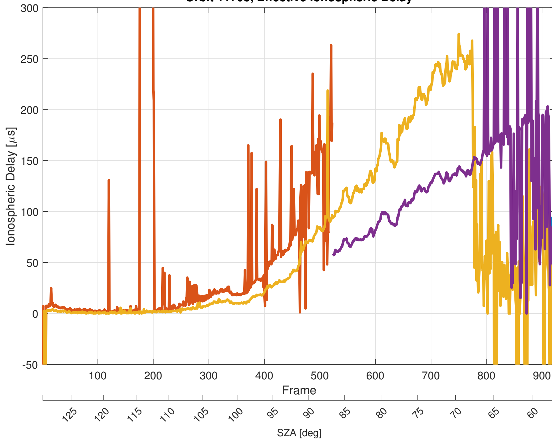
Orbit 11708, Effective Ionospheric Delay
