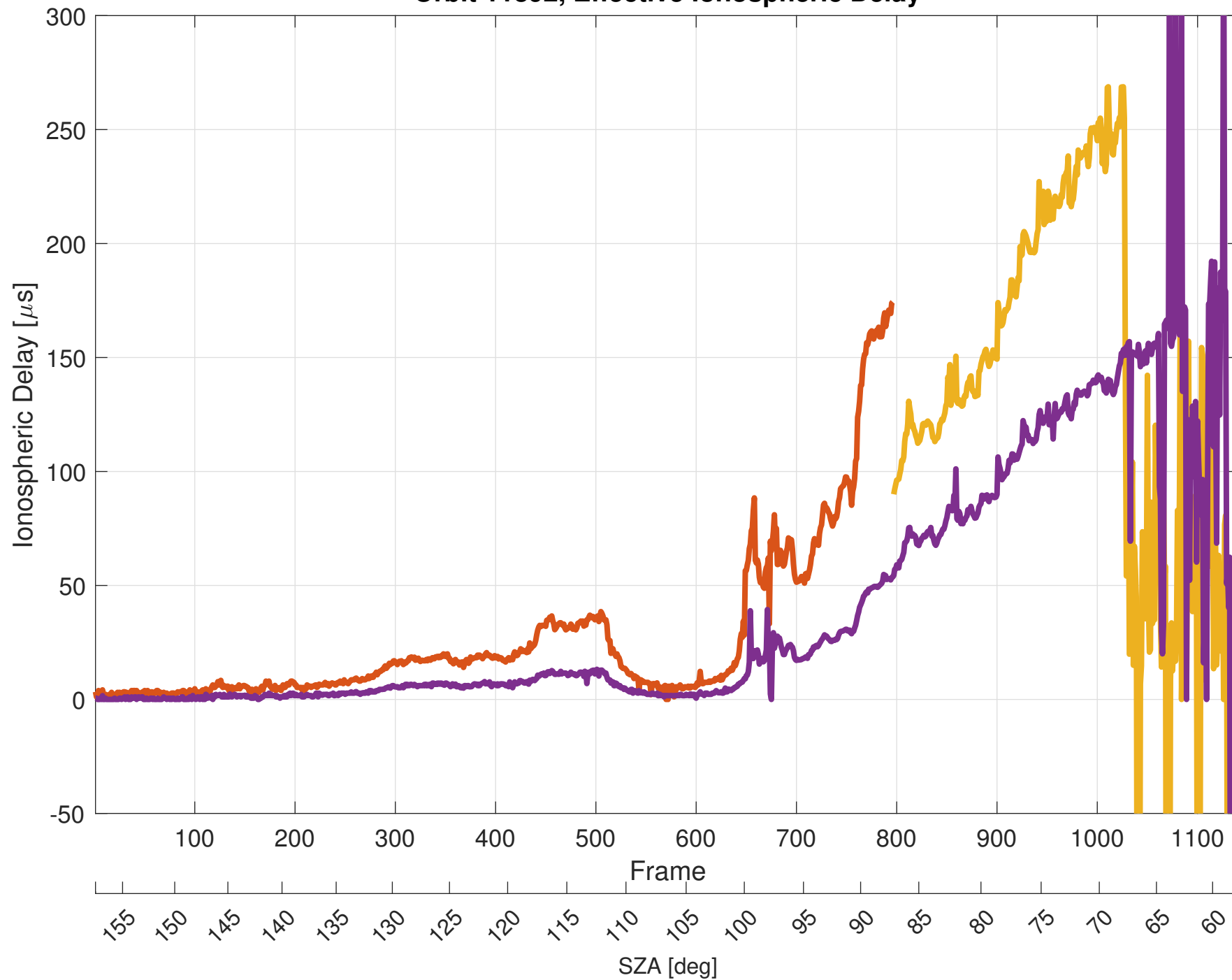
Orbit 11892, Effective Ionospheric Delay
