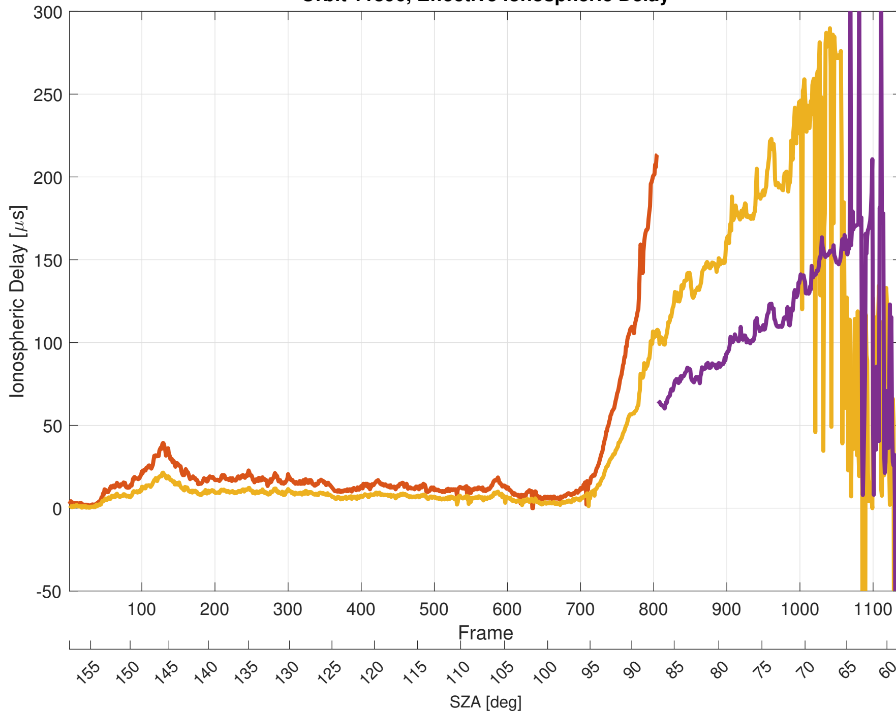
Orbit 11896, Effective Ionospheric Delay
