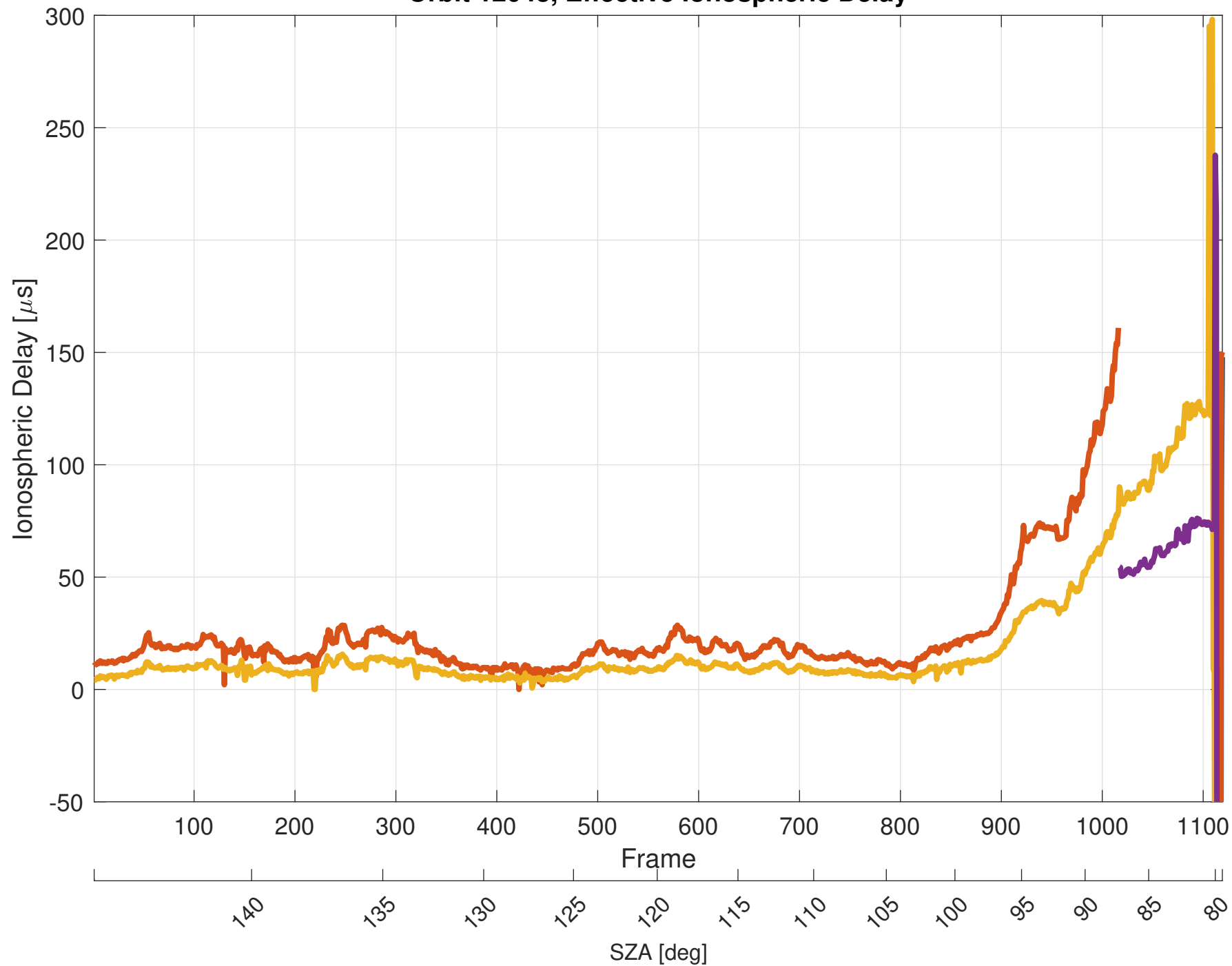
Orbit 12043, Effective Ionospheric Delay
