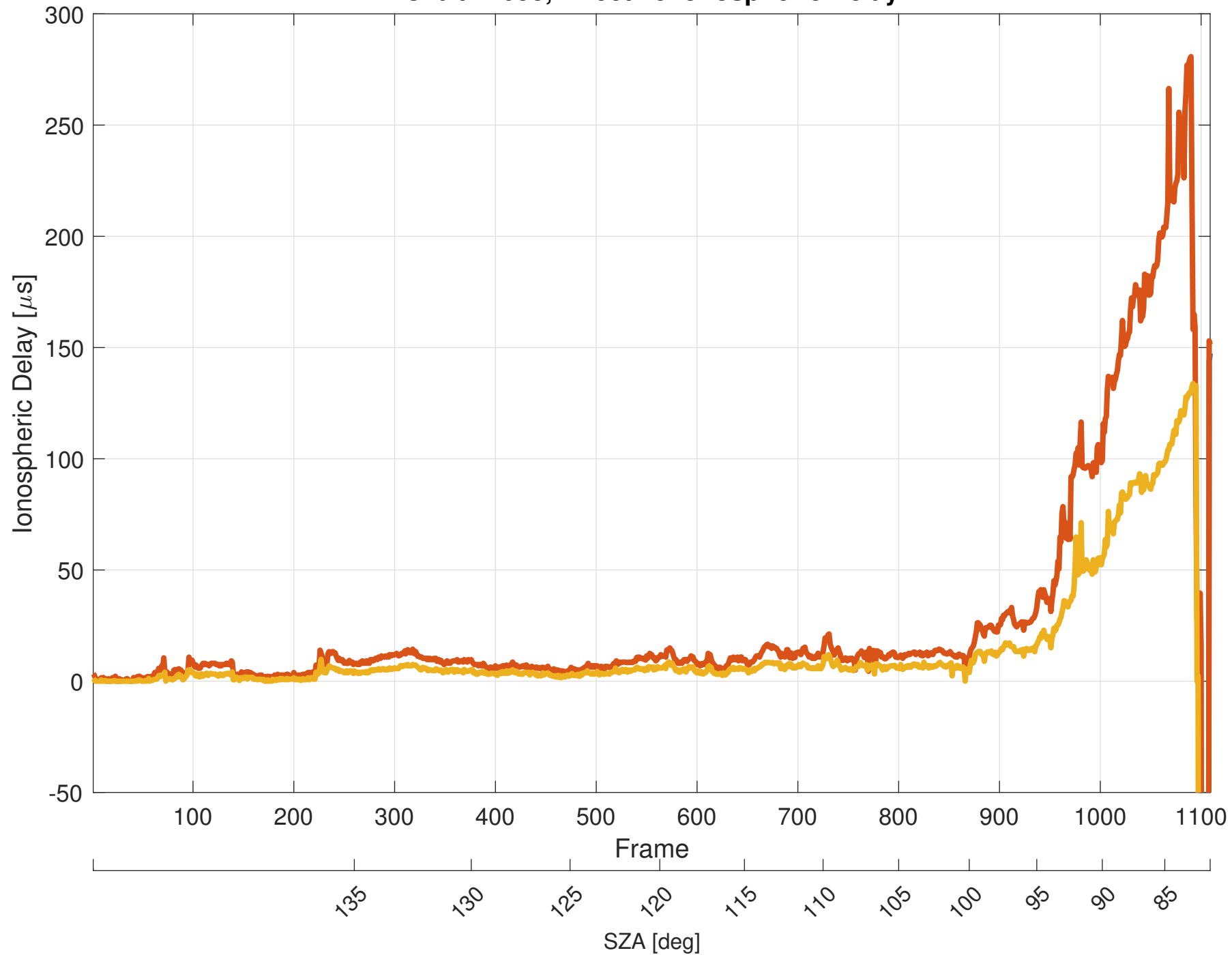
Orbit 12058, Effective Ionospheric Delay
