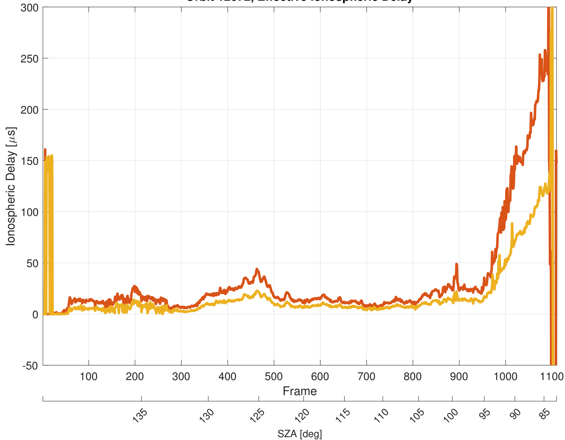
Orbit 12072, Effective Ionospheric Delay
