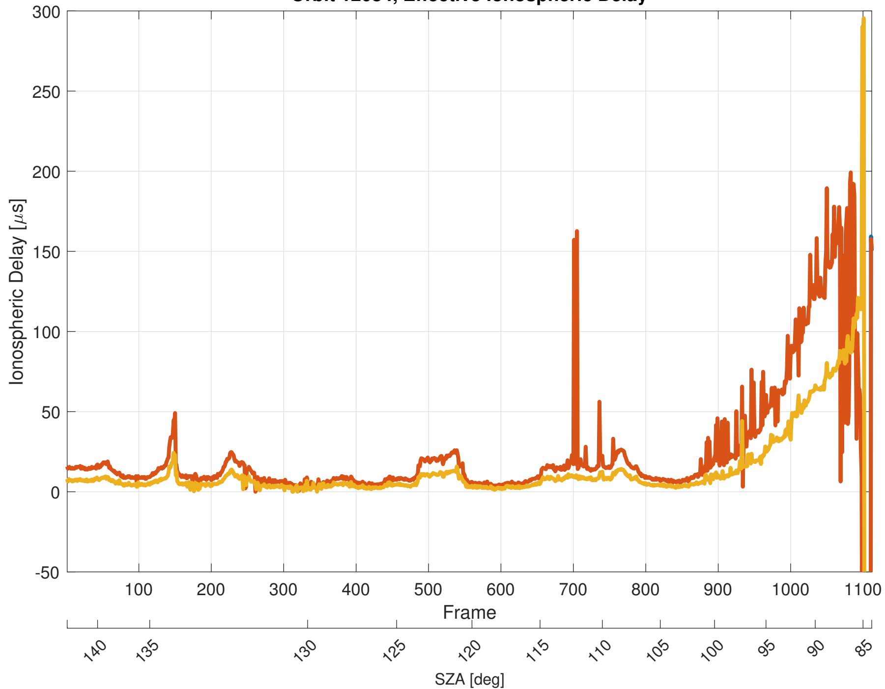
Orbit 12084, Effective Ionospheric Delay
