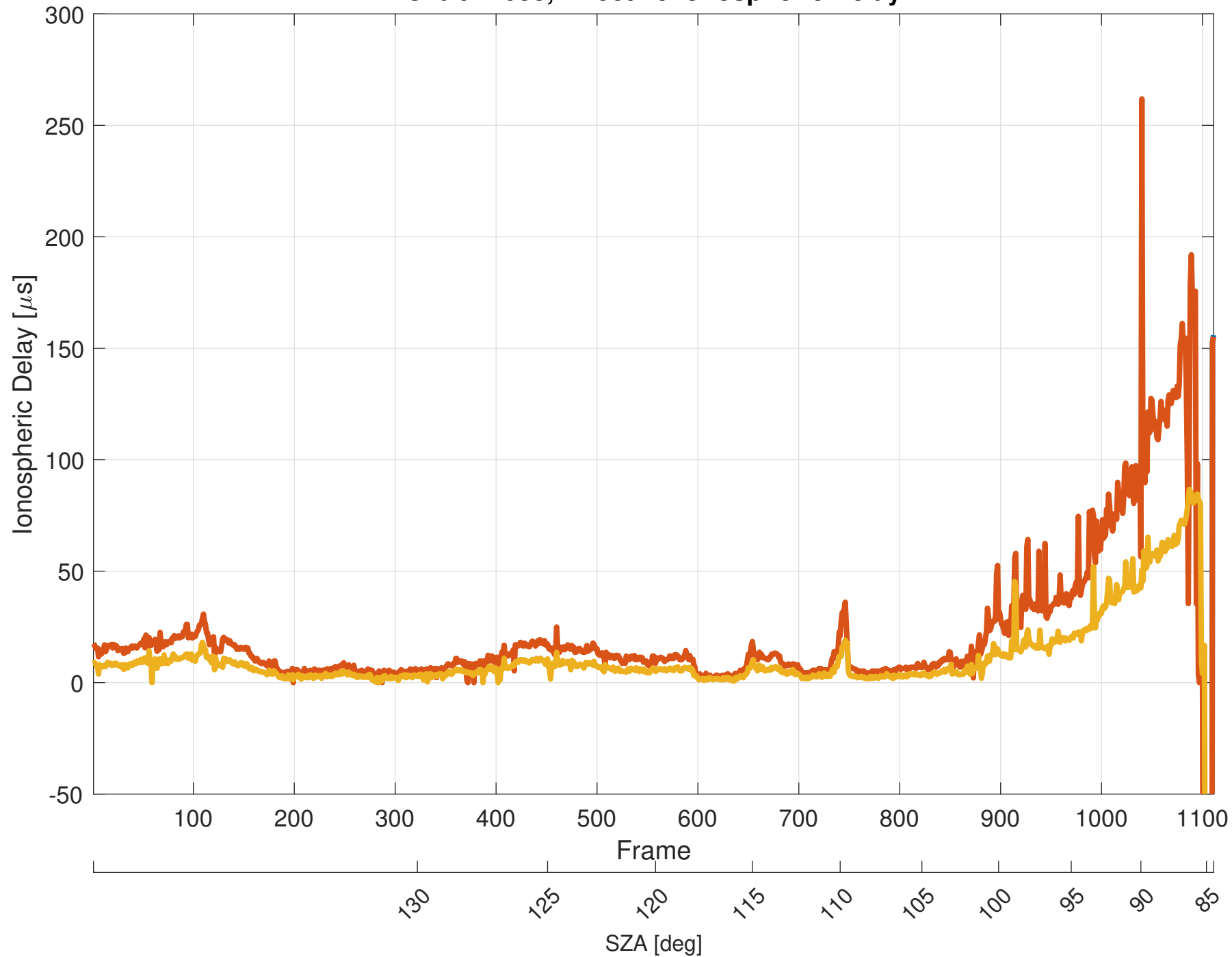
Orbit 12088, Effective Ionospheric Delay
