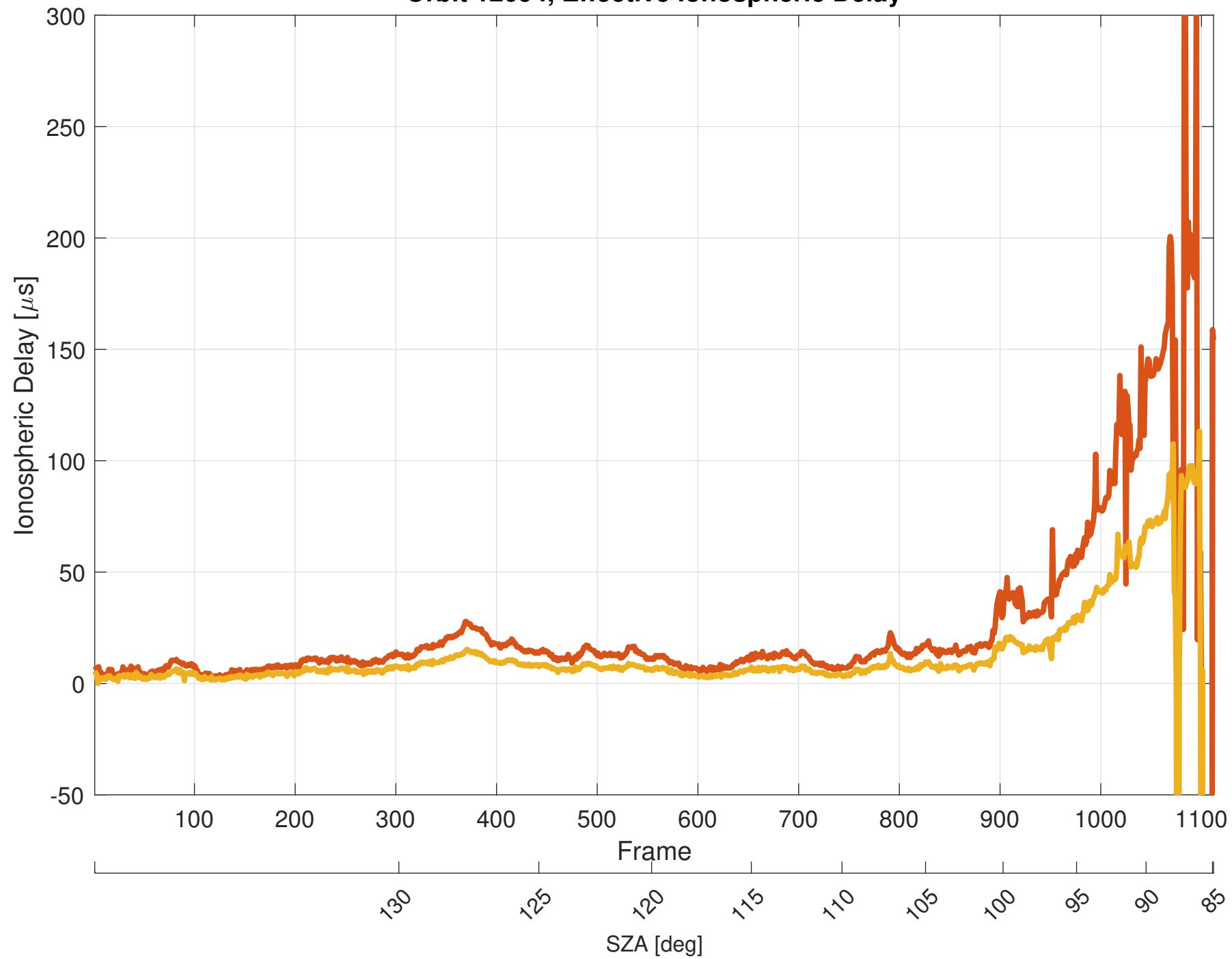
Orbit 12094, Effective Ionospheric Delay
