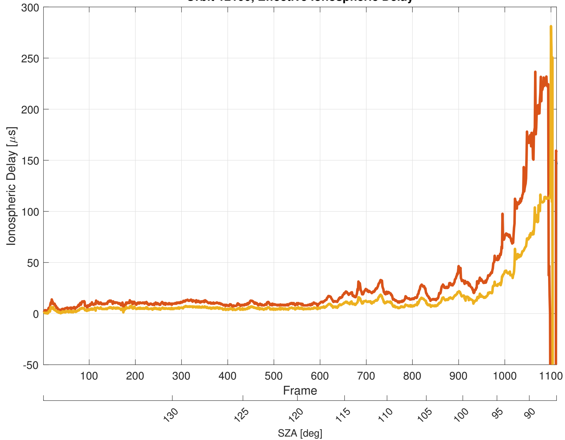
Orbit 12100, Effective Ionospheric Delay
