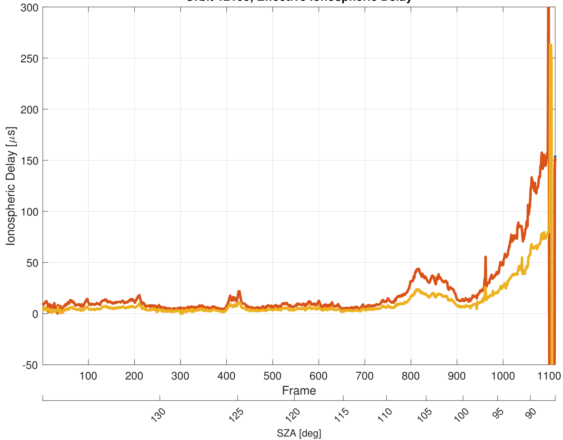
Orbit 12105, Effective Ionospheric Delay
