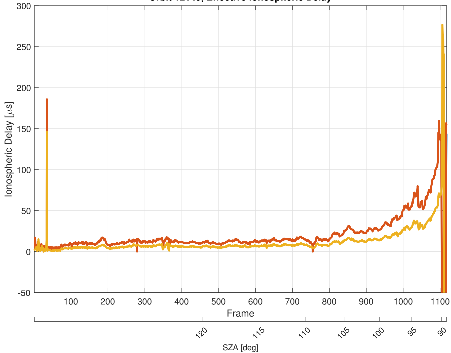
Orbit 12149, Effective Ionospheric Delay
