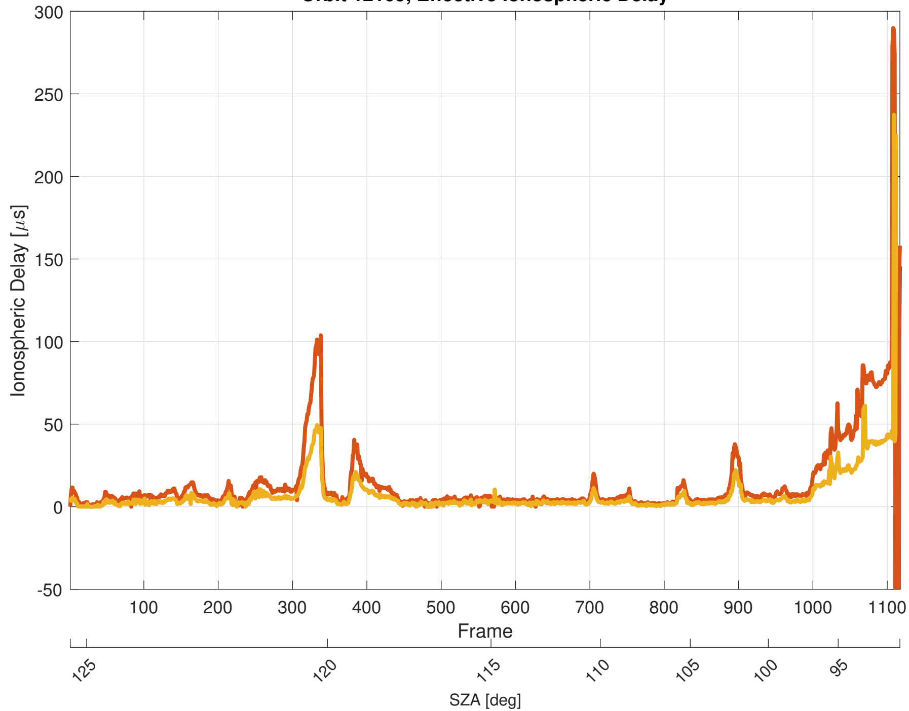
Orbit 12169, Effective Ionospheric Delay
