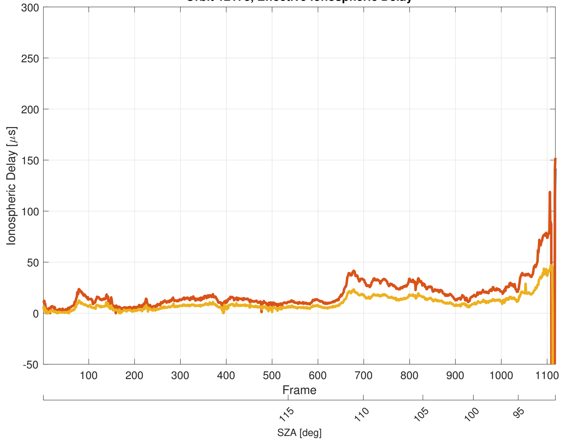
Orbit 12178, Effective Ionospheric Delay
