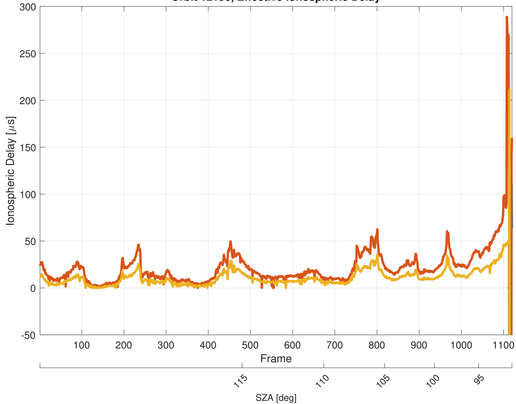
Orbit 12190, Effective Ionospheric Delay
