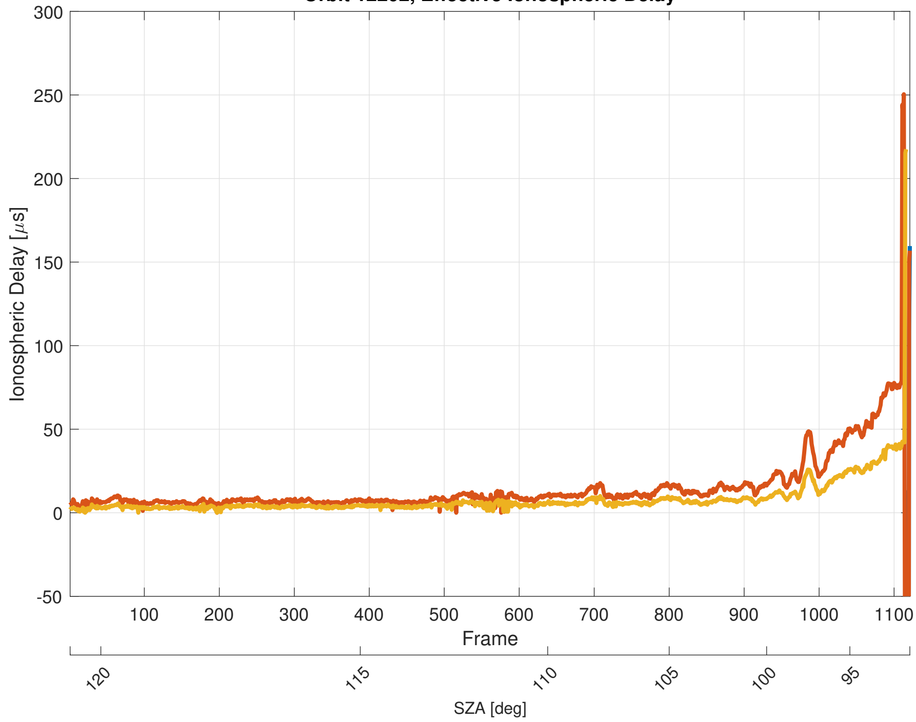
Orbit 12202, Effective Ionospheric Delay
