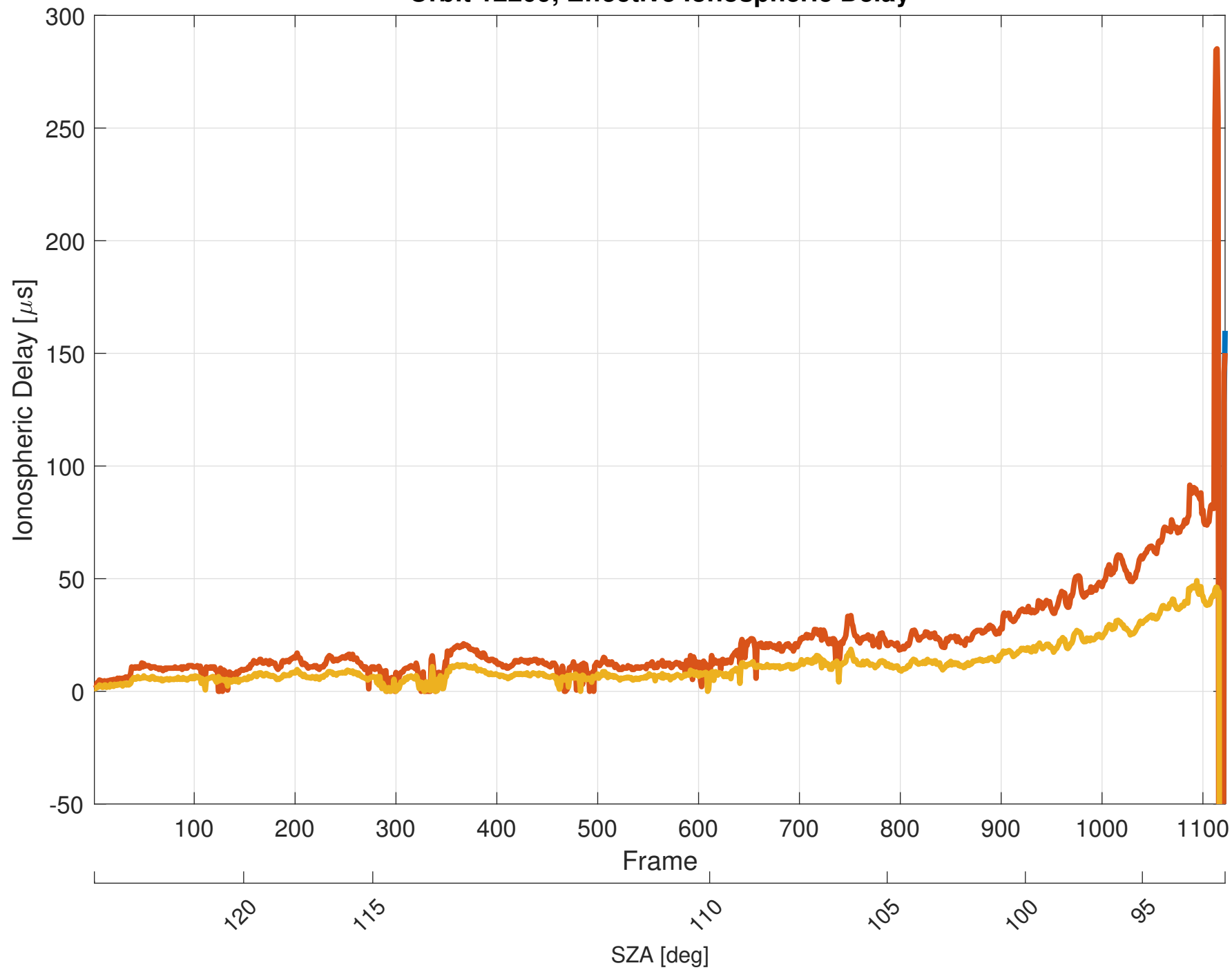
Orbit 12209, Effective Ionospheric Delay
