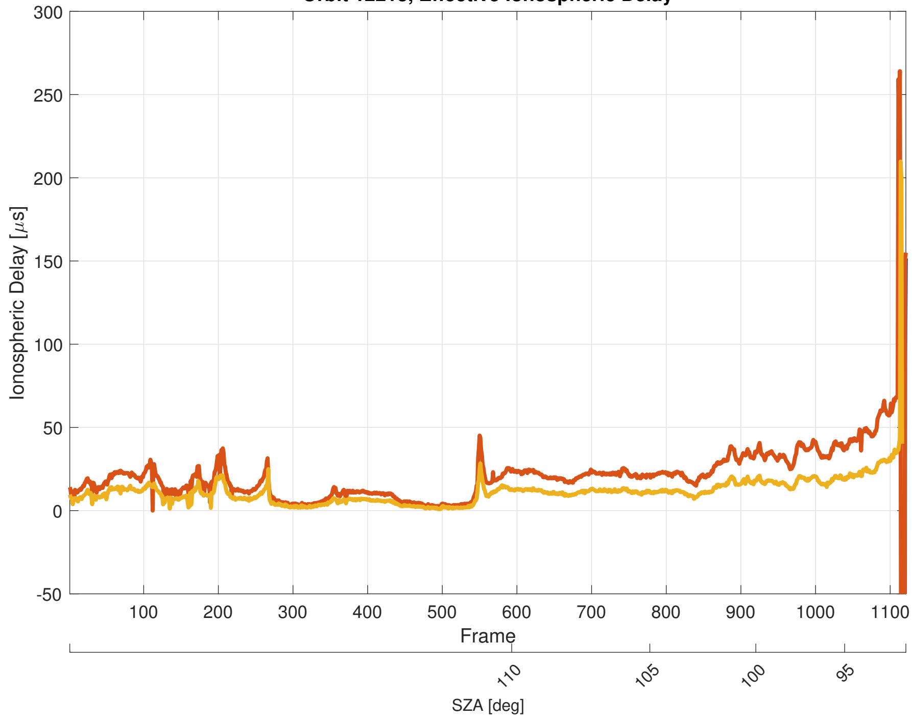
Orbit 12213, Effective Ionospheric Delay
