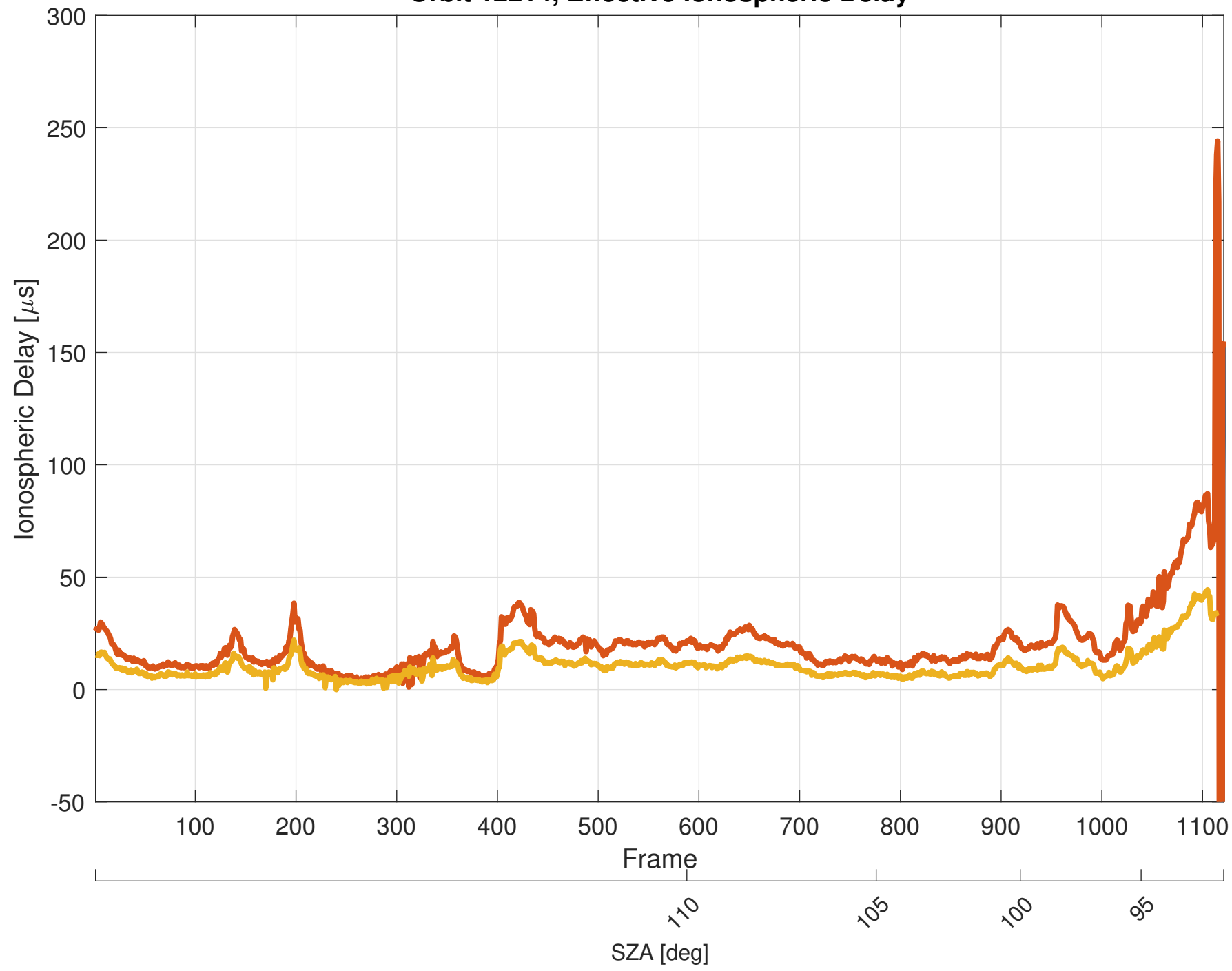
Orbit 12214, Effective Ionospheric Delay
