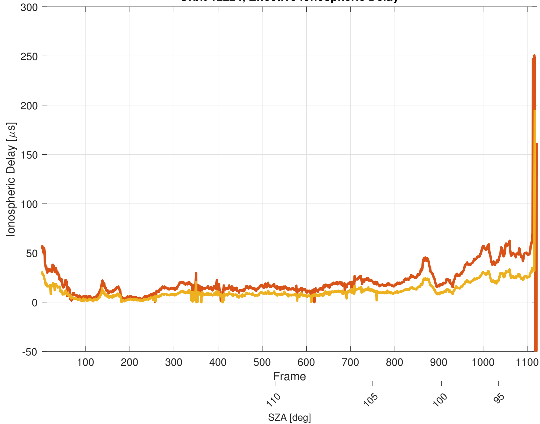
Orbit 12224, Effective Ionospheric Delay
