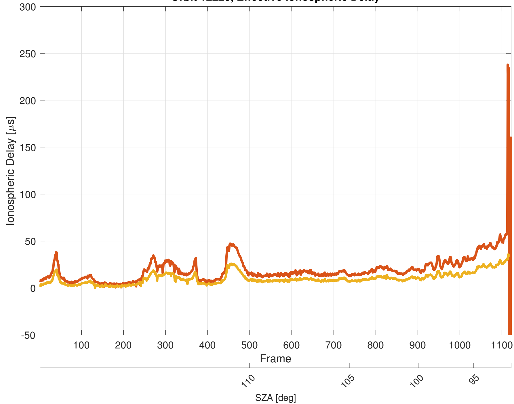
Orbit 12228, Effective Ionospheric Delay
