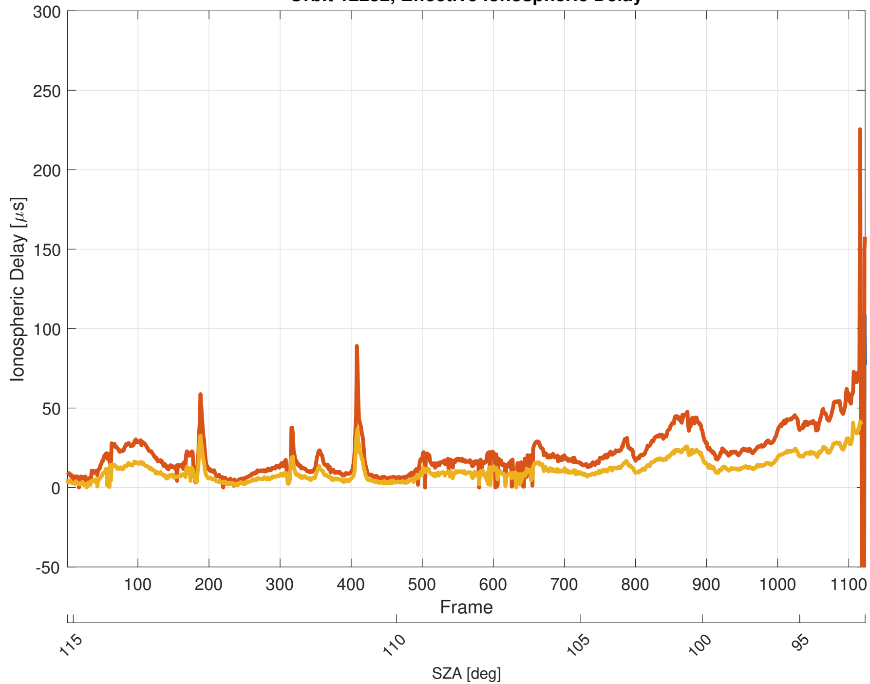
Orbit 12232, Effective Ionospheric Delay
