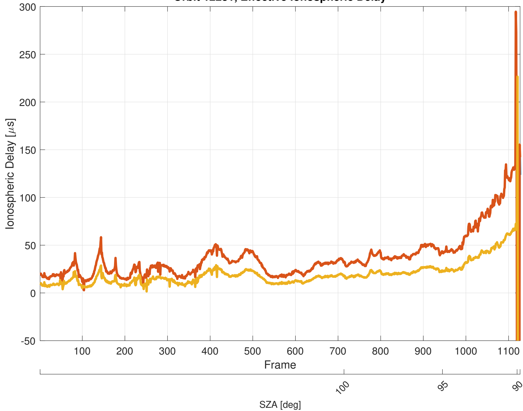
Orbit 12281, Effective Ionospheric Delay
