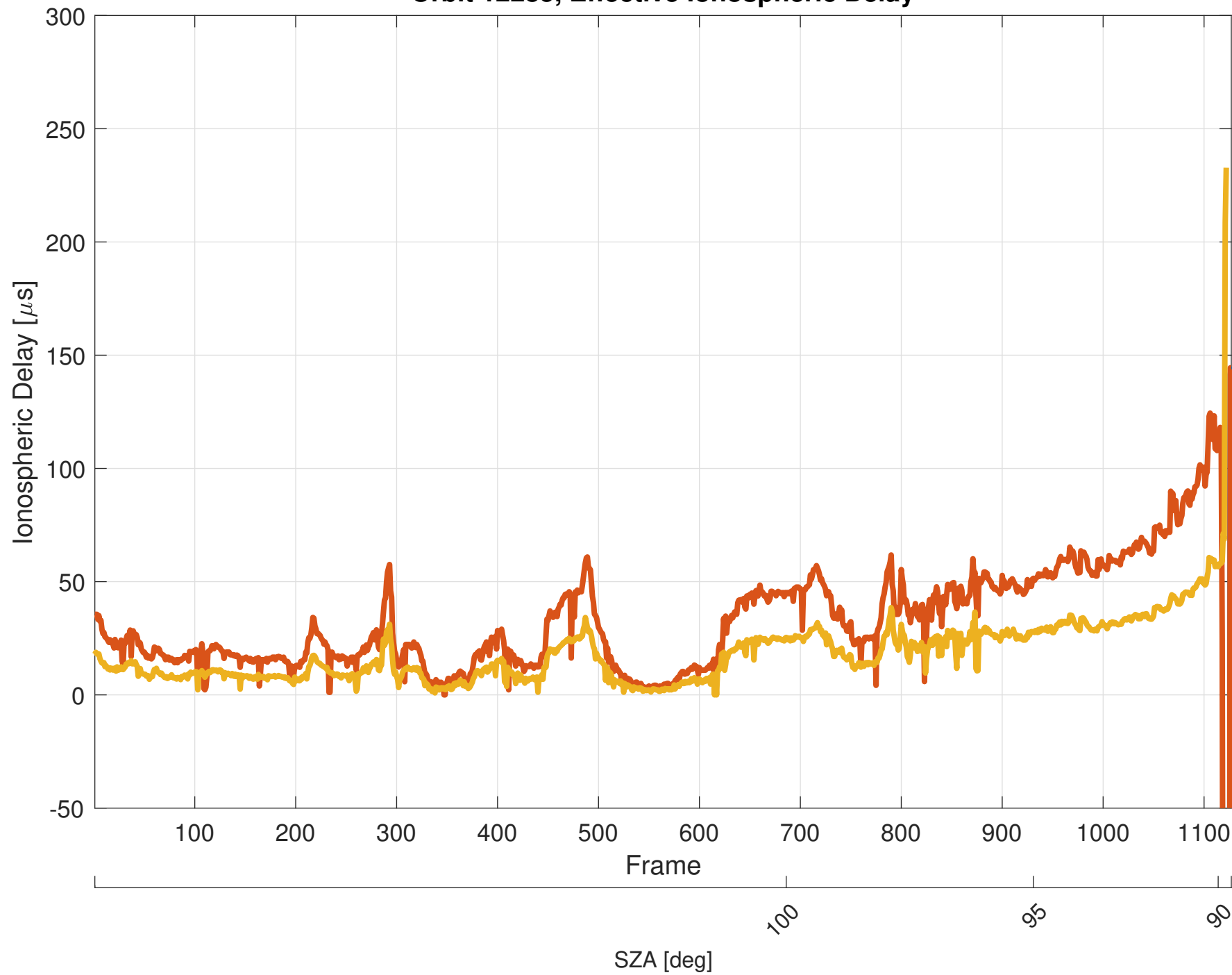
Orbit 12285, Effective Ionospheric Delay
