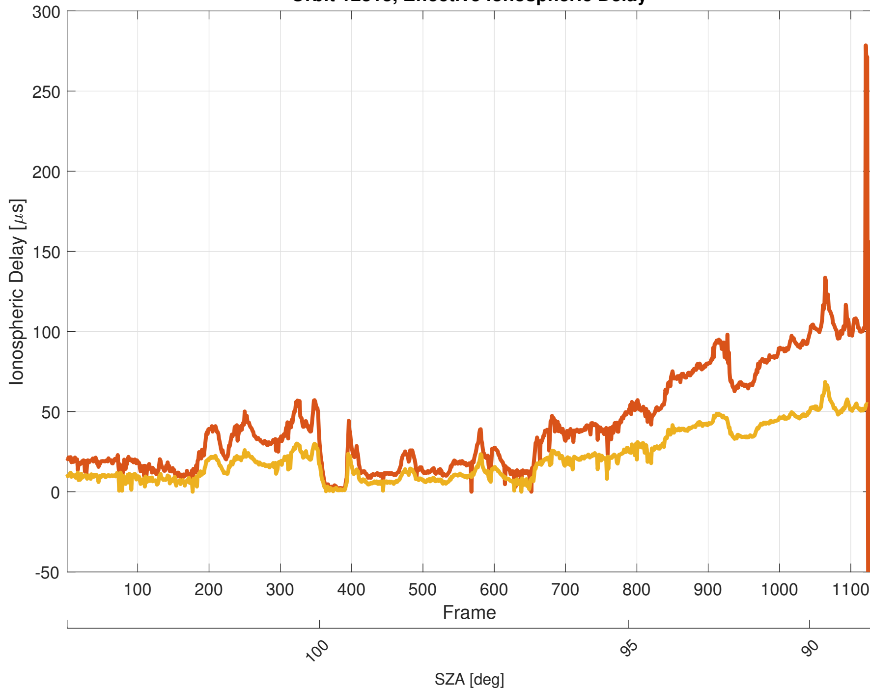
Orbit 12313, Effective Ionospheric Delay
