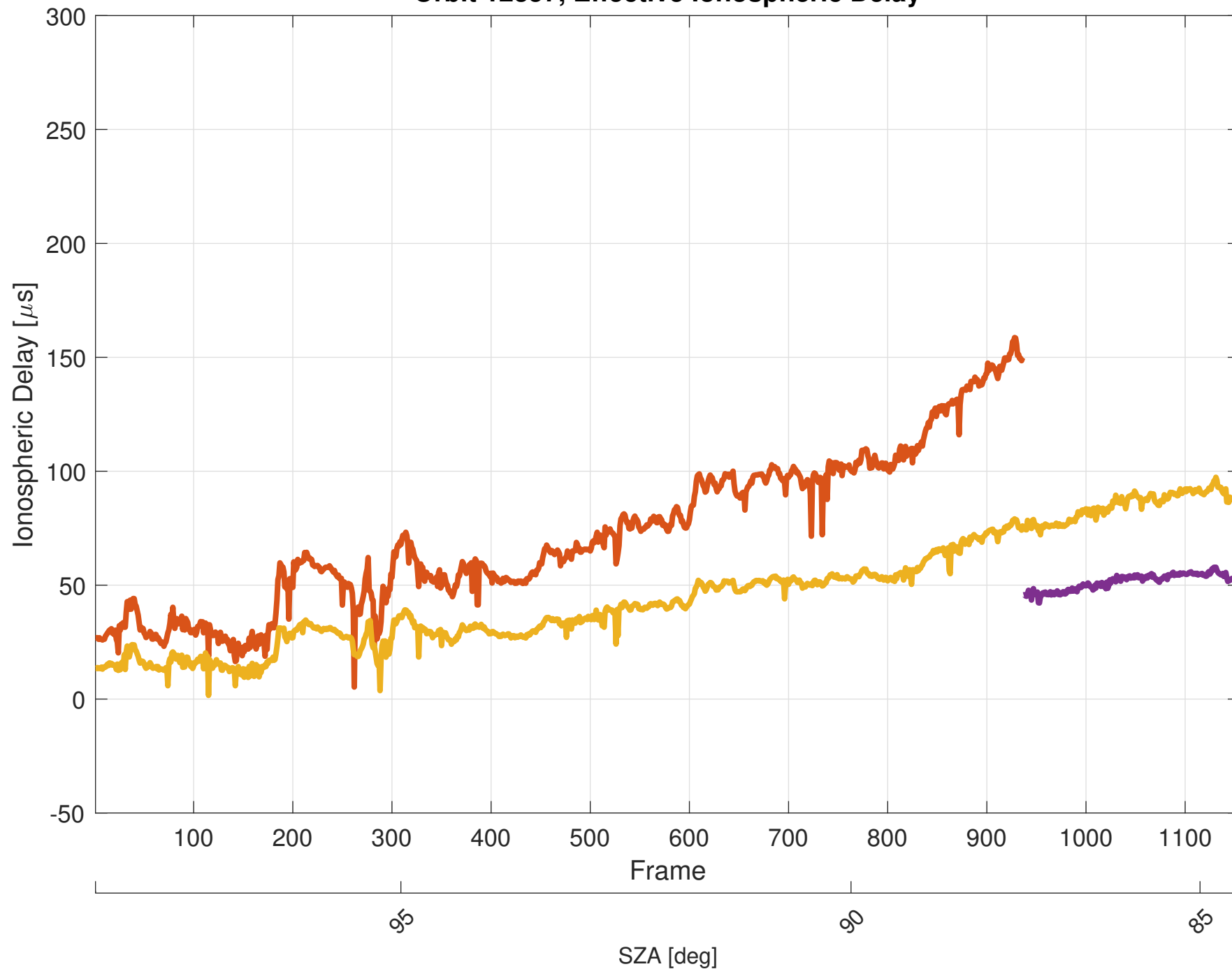
Orbit 12357, Effective Ionospheric Delay
