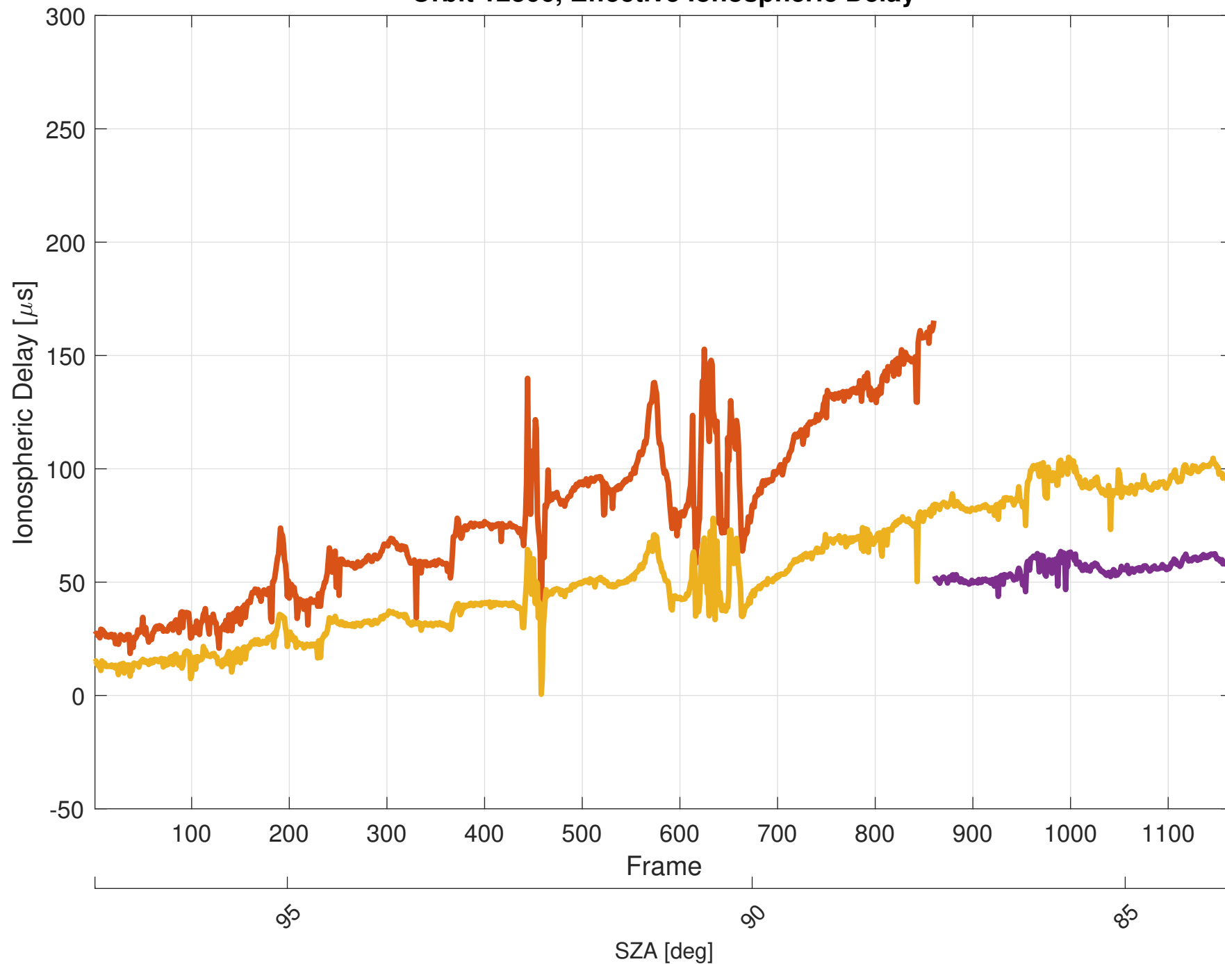
Orbit 12366, Effective Ionospheric Delay
