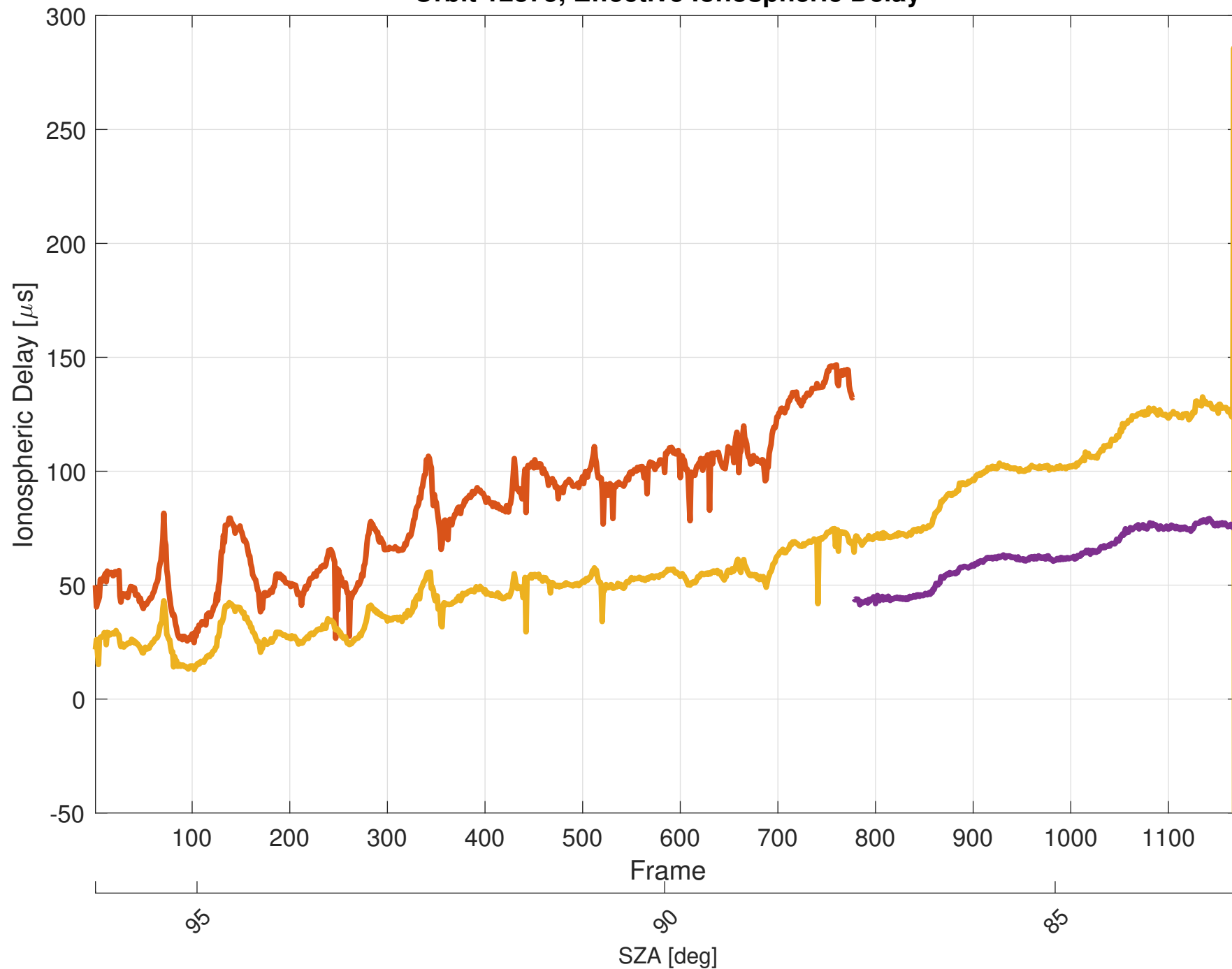
Orbit 12375, Effective Ionospheric Delay
