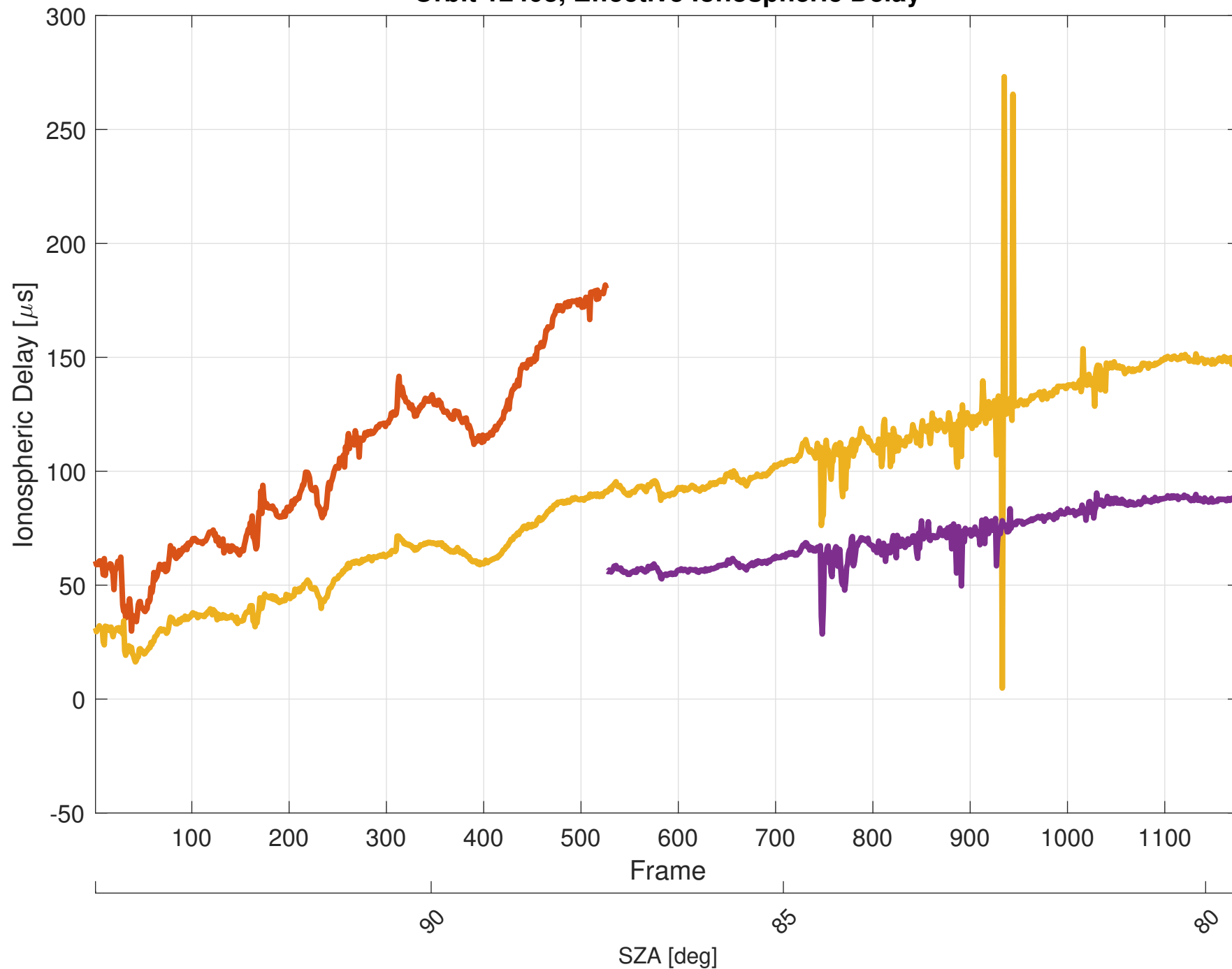
Orbit 12403, Effective Ionospheric Delay
