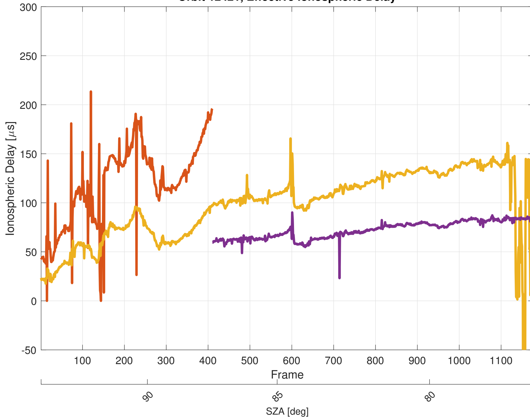
Orbit 12421, Effective Ionospheric Delay
