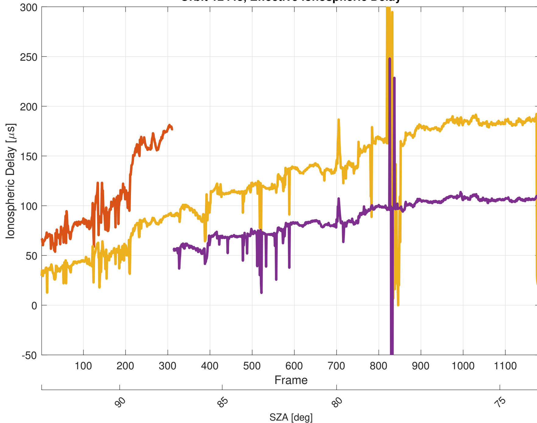
Orbit 12448, Effective Ionospheric Delay
