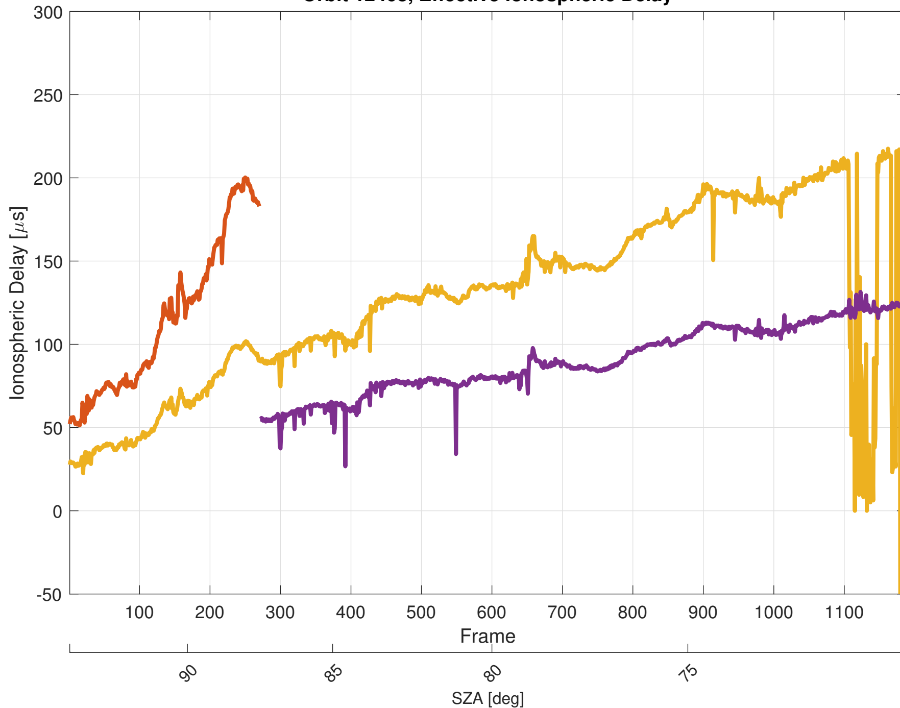
Orbit 12468, Effective Ionospheric Delay
