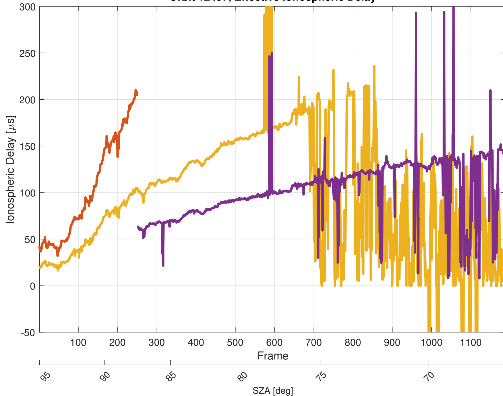
Orbit 12497, Effective Ionospheric Delay
