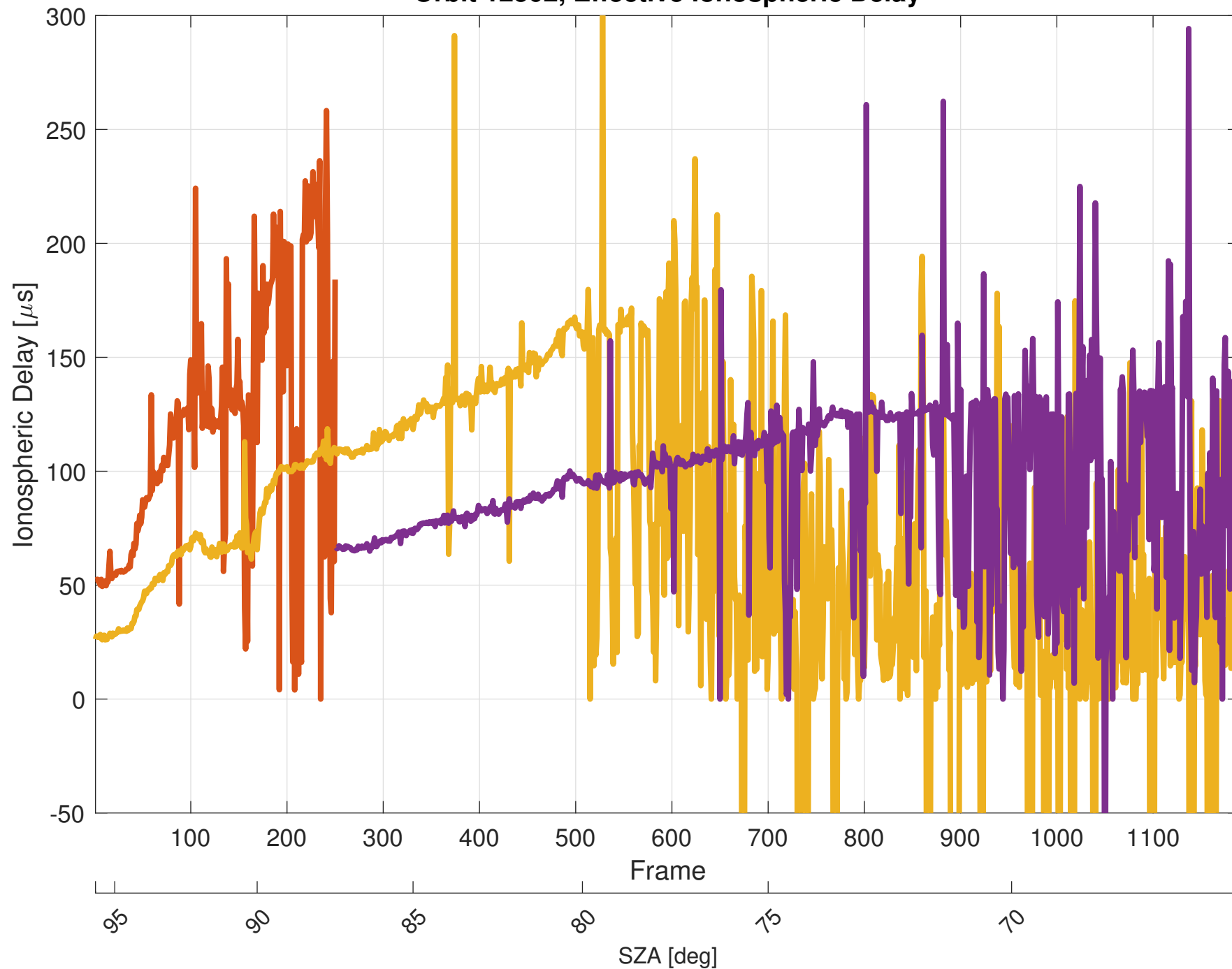
Orbit 12502, Effective Ionospheric Delay
