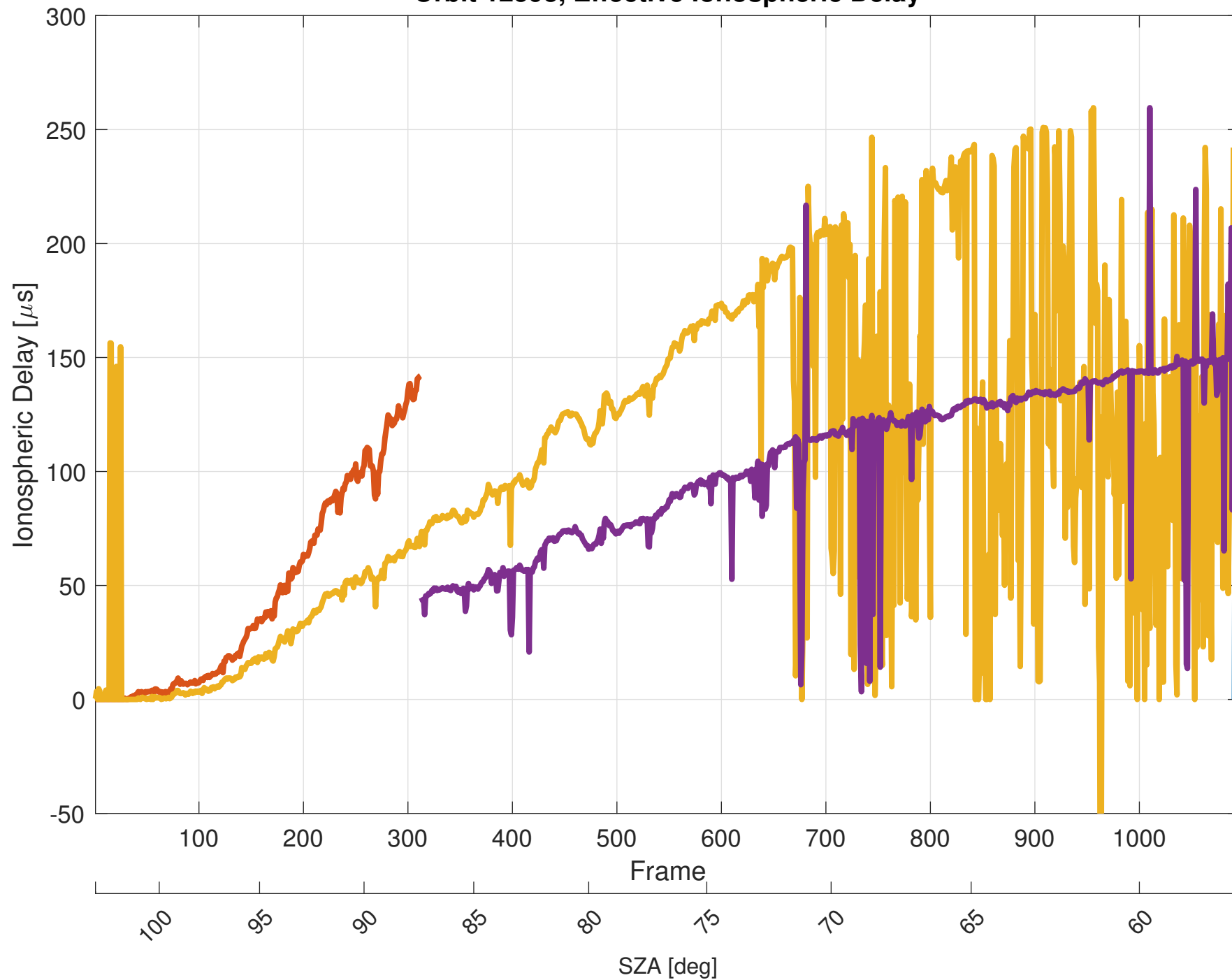
Orbit 12593, Effective Ionospheric Delay
