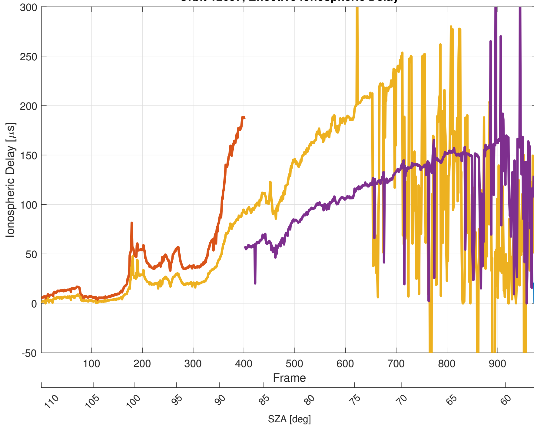
Orbit 12657, Effective Ionospheric Delay
