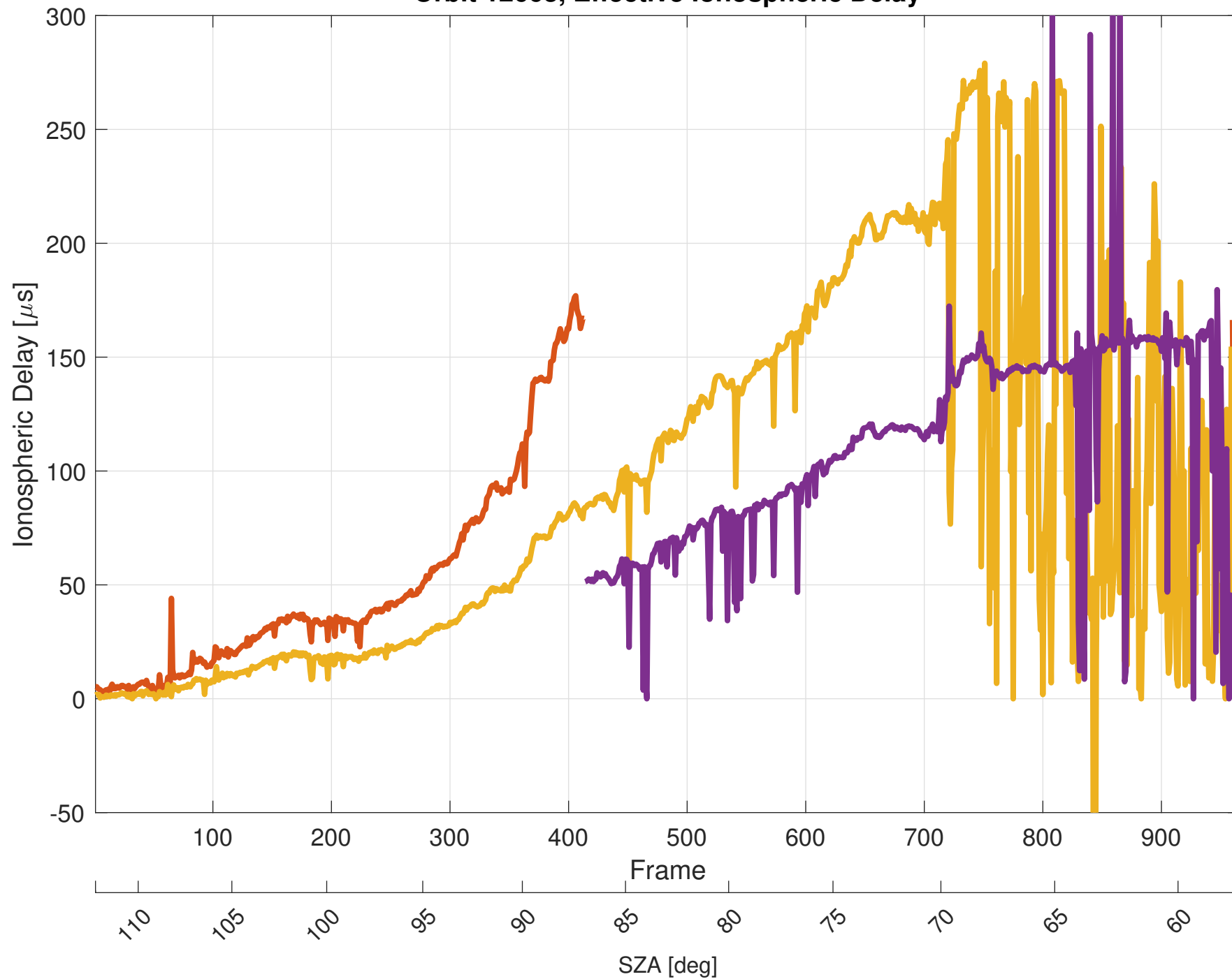
Orbit 12663, Effective Ionospheric Delay
