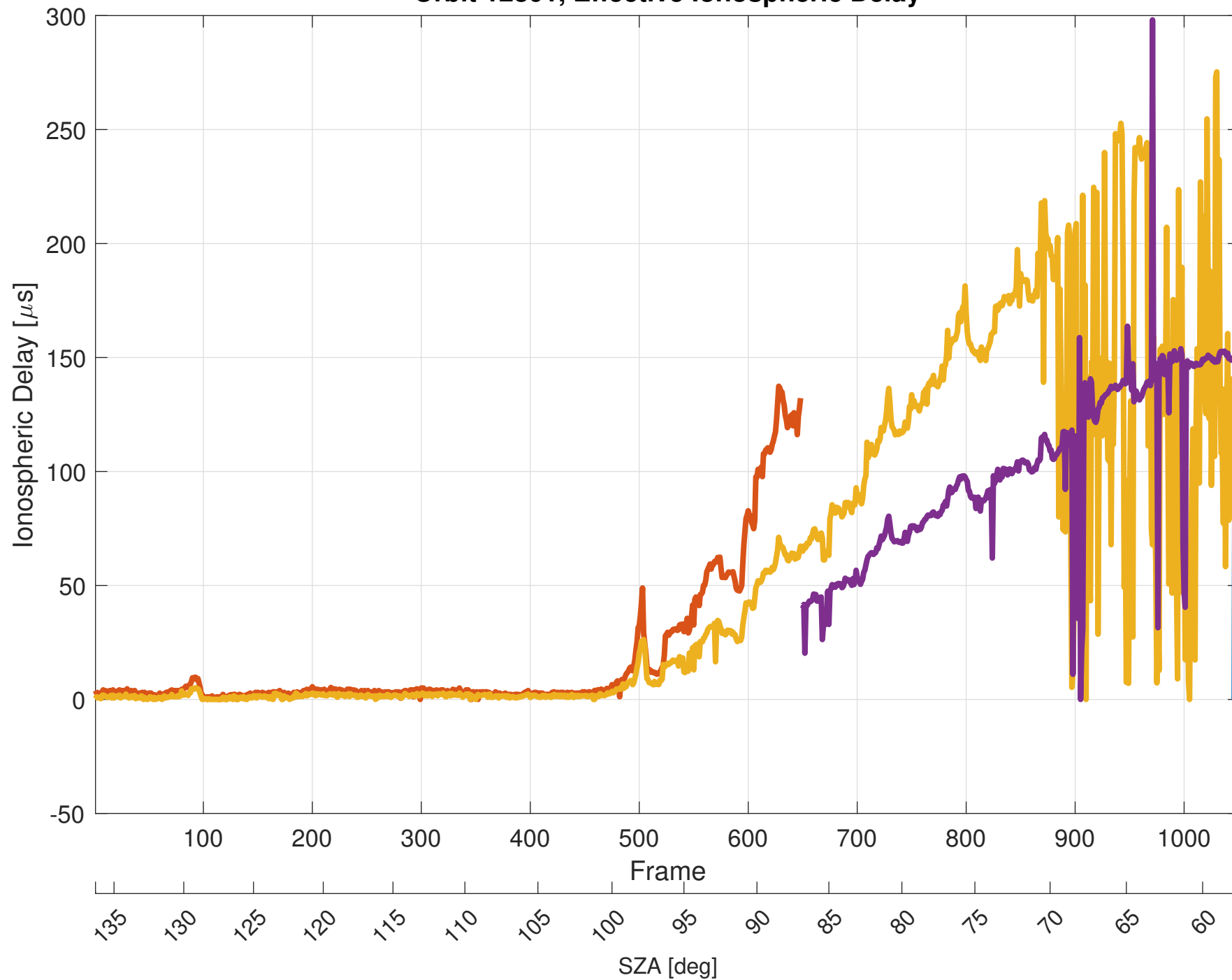
Orbit 12801, Effective Ionospheric Delay
